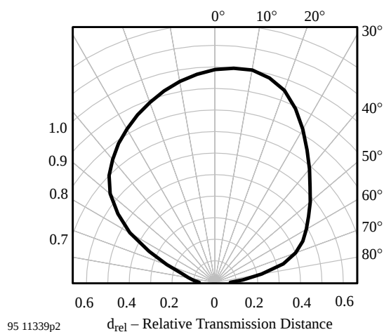
Figure 13. Vertical Directivity \phi_V
