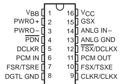
TCM29C16, TCM29C17, TCM129C16, TCM129C17 DW OR N PACKAGE (TOP VIEW)
