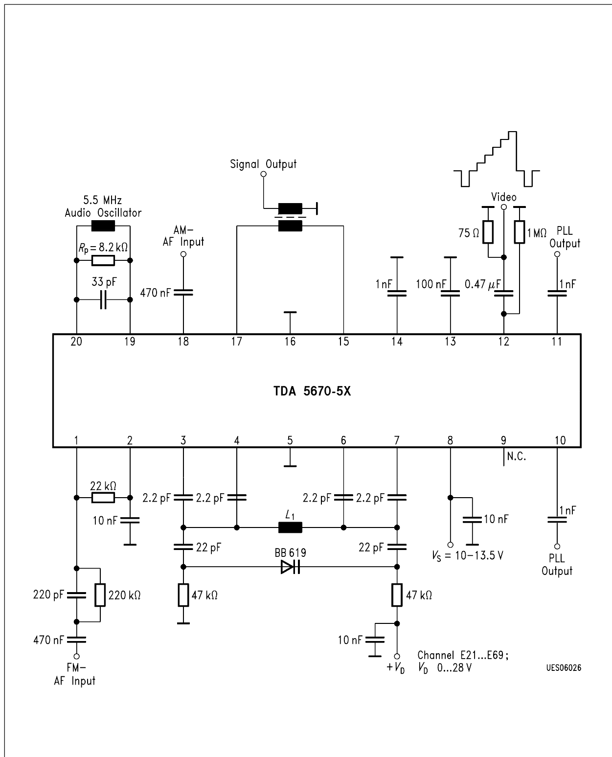
Application Circuit
