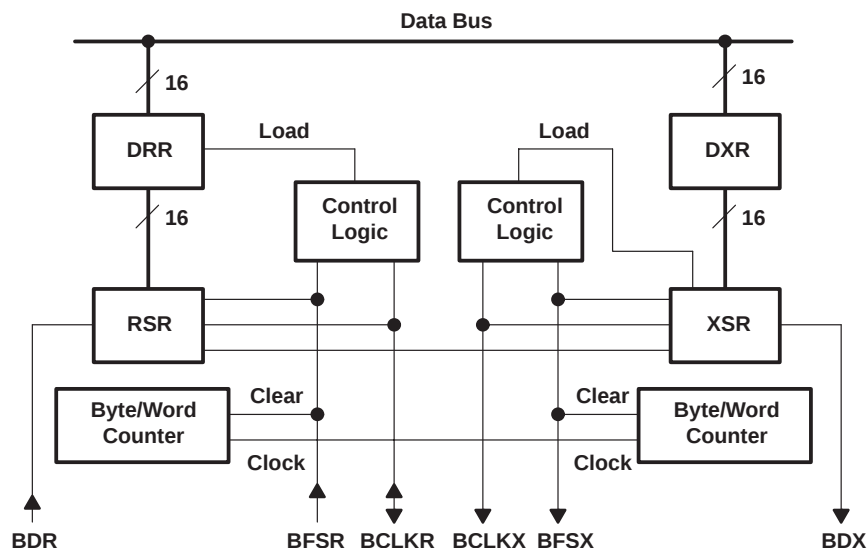
Figure 16. DSP Serial Digital Interface
