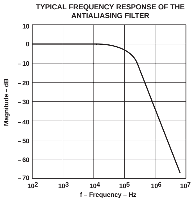
Figure 8. Antialiasing Filter
