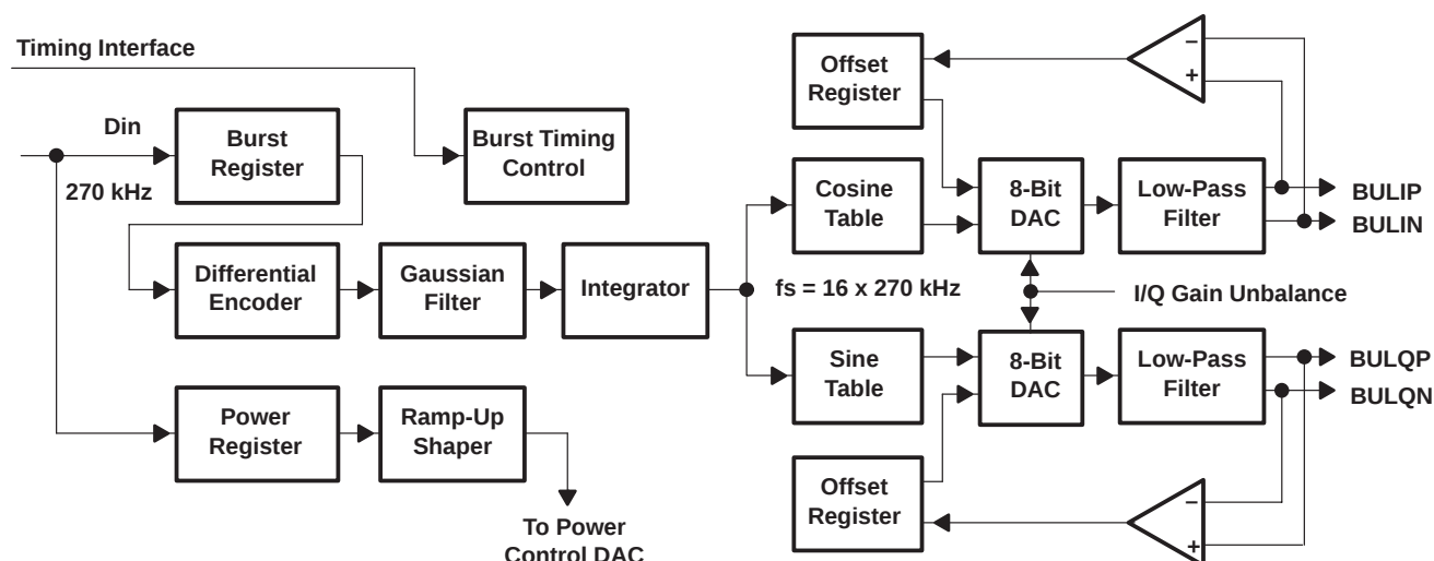
Figure 7. Functional Structure Of The Baseband Uplink Path
