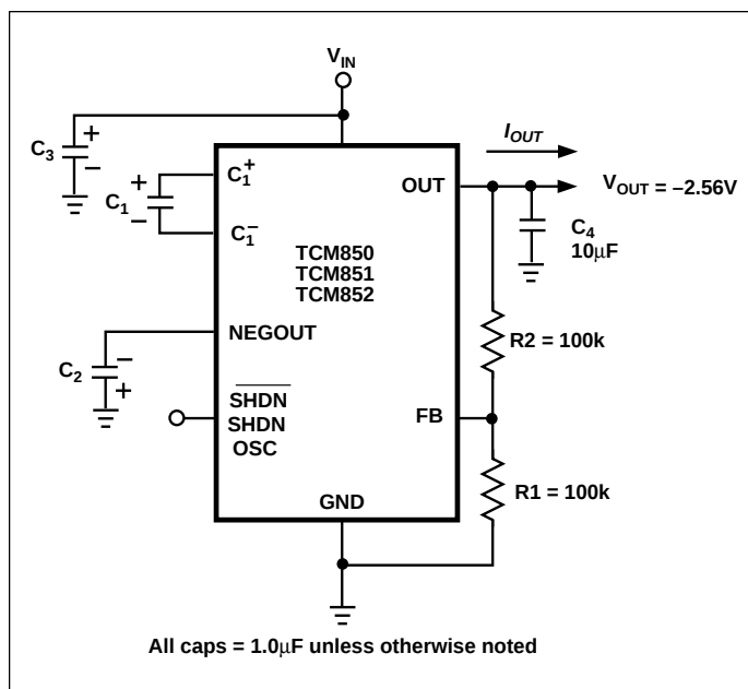
Figure 4. TCM850/851/852 Adjustable Application
