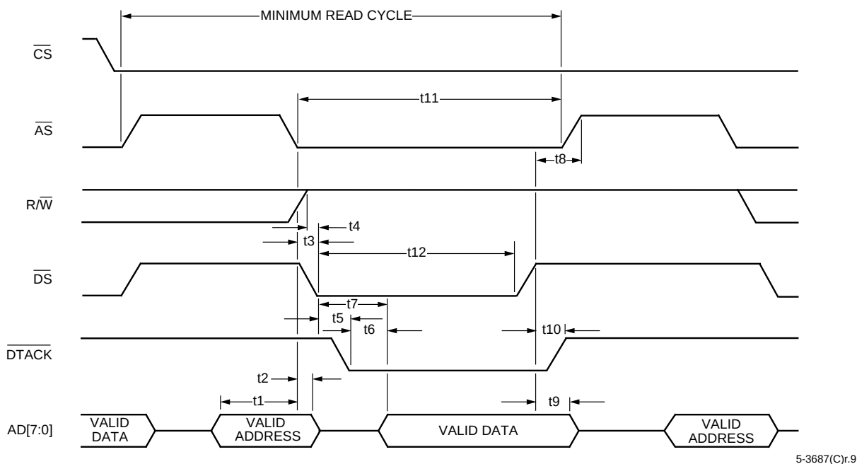
Figure 6. Mode2—Read Cycle Timing (MPPMODE = 0, MPMUX = 1)
