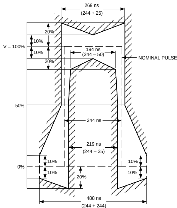
Figure 3. ITU-T G.703 Pulse Template
