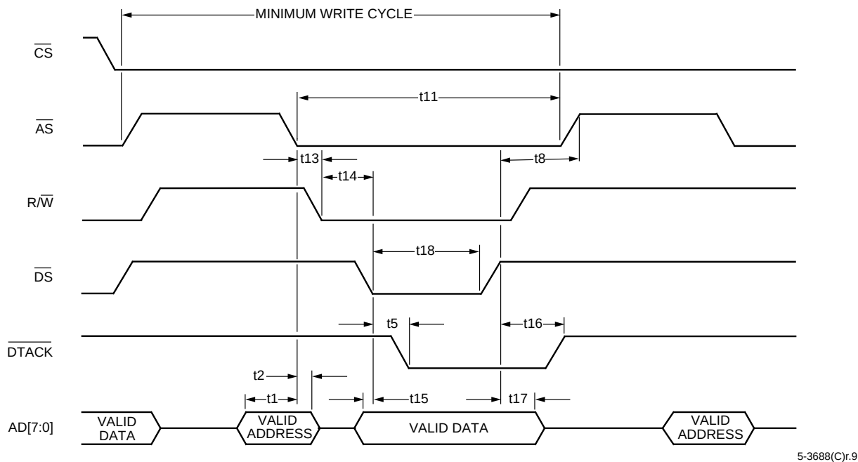
Figure 7. Mode2—Write Cycle Timing (MPPMODE = 0, MPMUX = 1)
