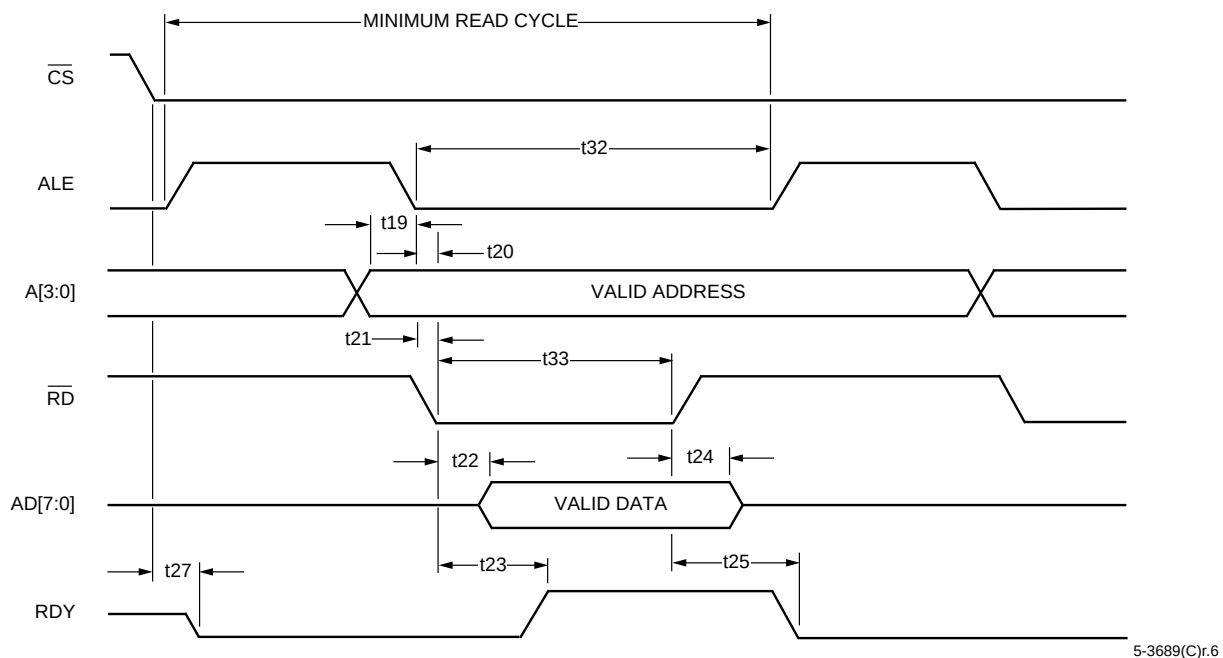
Figure 8. Mode3—Read Cycle Timing (MPMODE = 1, MPMUX = 0)
