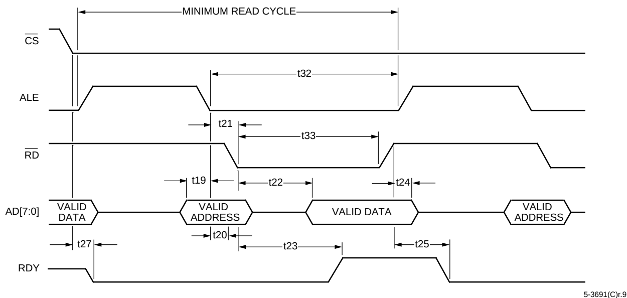
Figure 10. Mode4—Read Cycle Timing (MPMODE = 1, MPMUX = 1)
