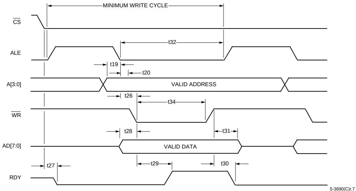
Figure 9. Mode3—Write Cycle Timing (MPMODE = 1, MPMUX = 0)
