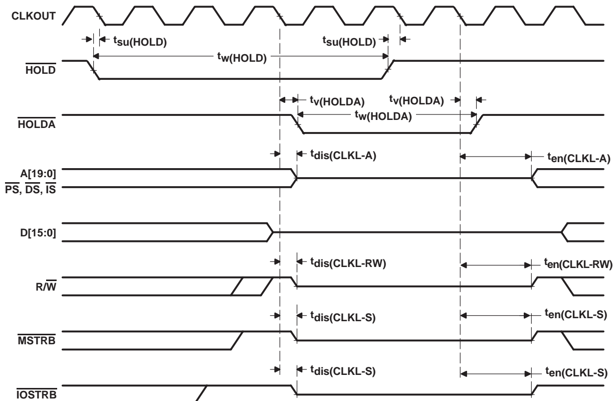
Figure 24. HOLD and HOLDA Timings (HM = 1)
