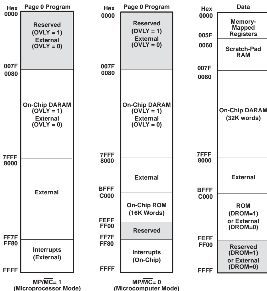
Figure 1. Memory Map
