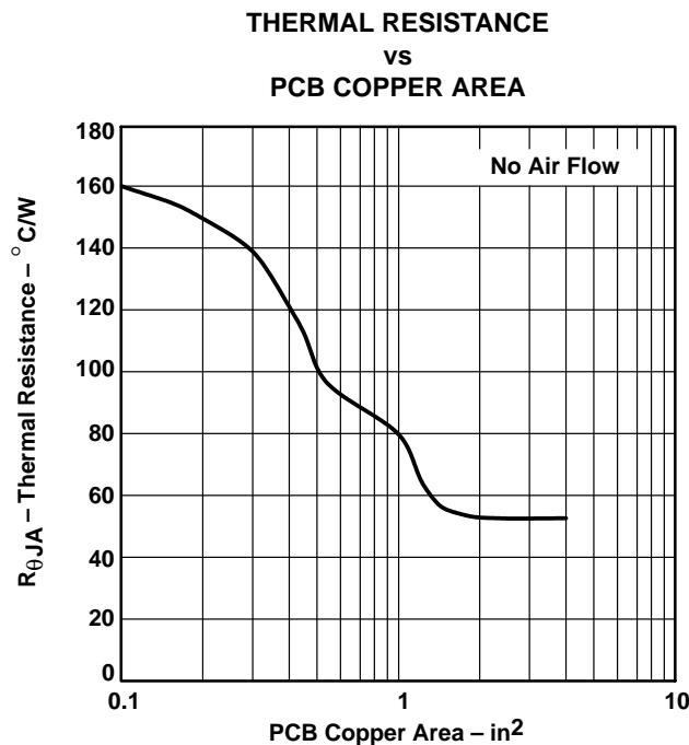
Figure 29. SOT223 Thermal Resistance vs PCB AREA
