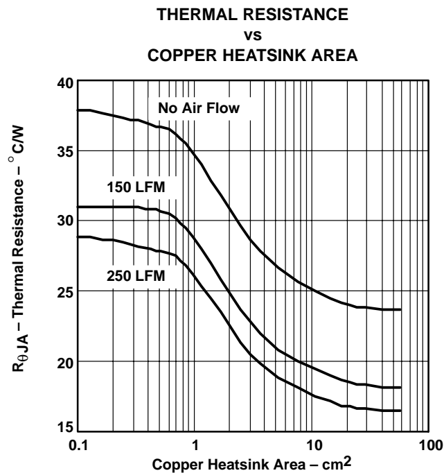
Figure 26. DDPACK Thermal Resistance vs Copper Heatsink Area
