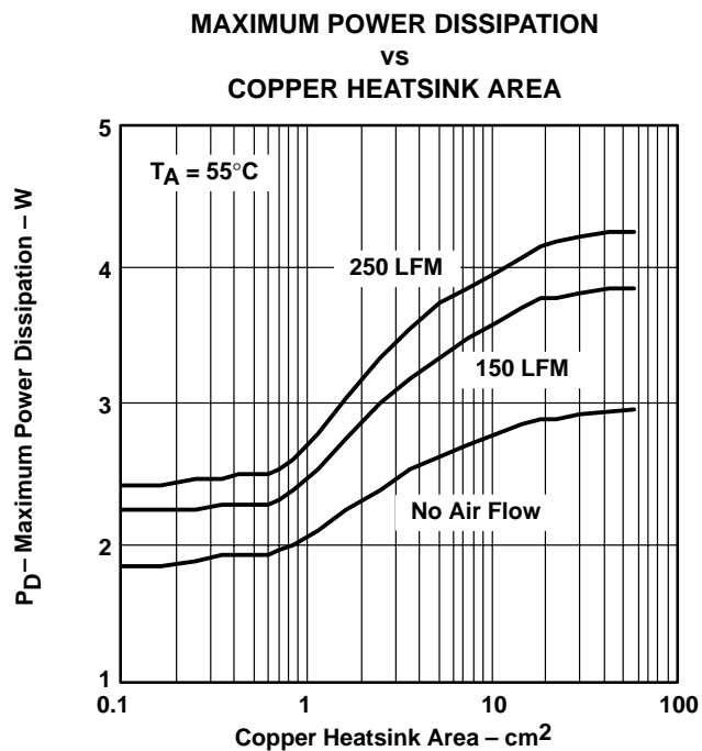
Figure 28. Maximum Power Dissipation vs Copper Heatsink Area
