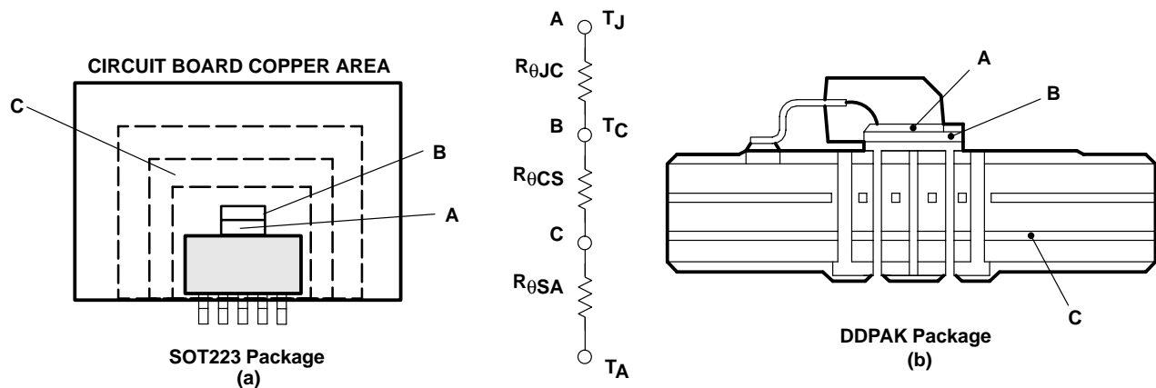
Figure 25. Thermal Resistances
