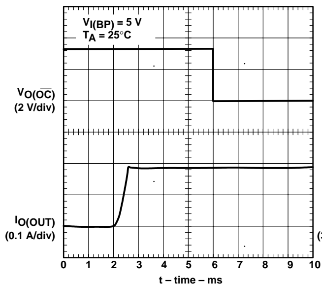
Figure 15. OC Response (BP Switch), Device Enabled Into Short
