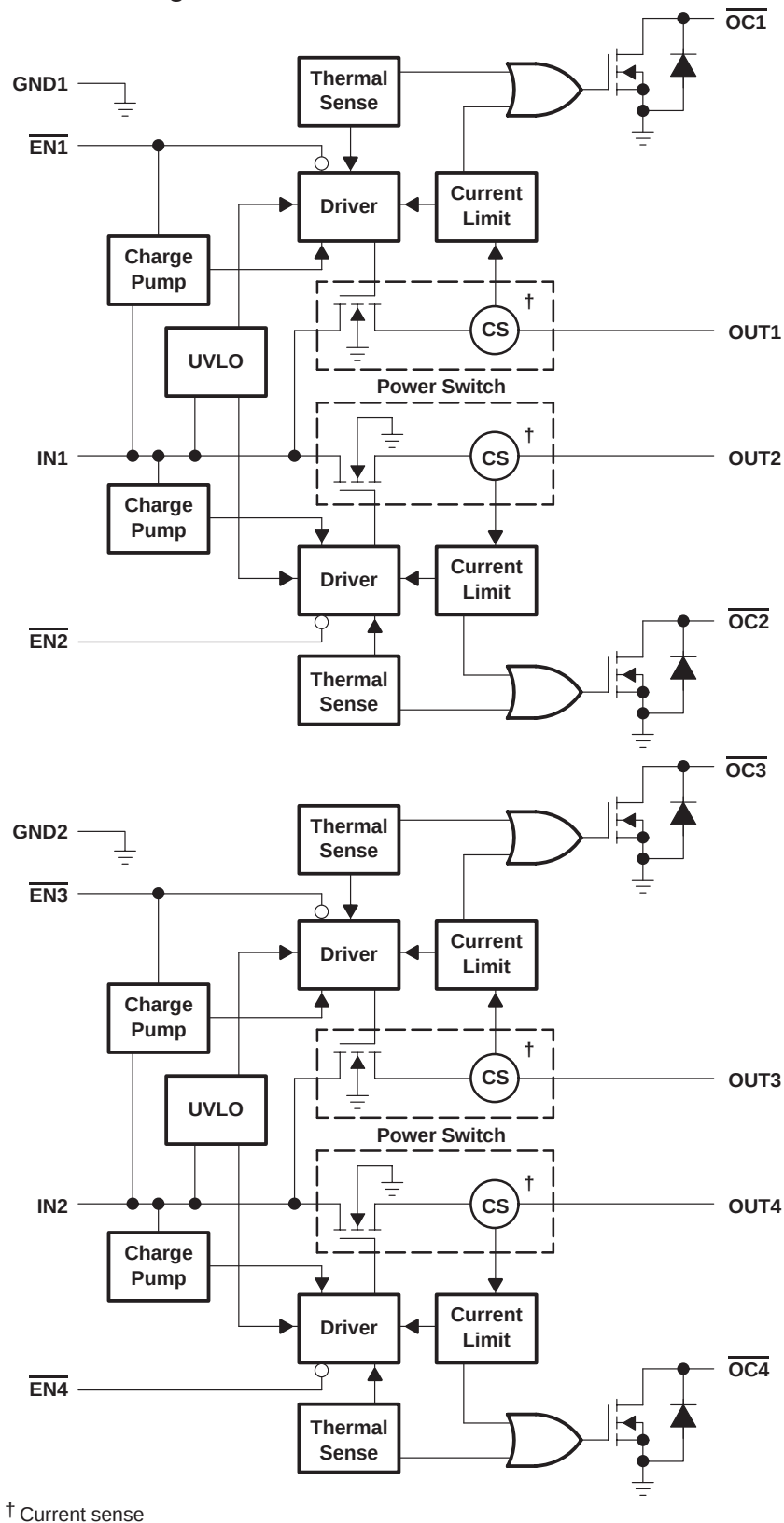
TPS2048 functional block diagram
