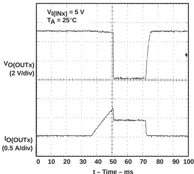
Figure 7. TPS2048, Threshold Trip Current with Ramped Load on Enabled Device
