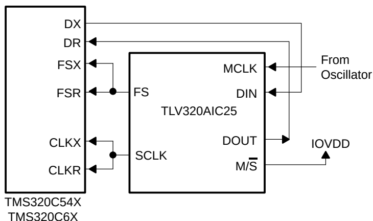
Figure 5–19. TLV320AIC25s Interface to McBSP Port of C54x or C6x DSP
