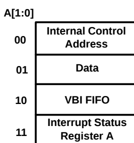
Figure 2–30. PHI Address Register Map
