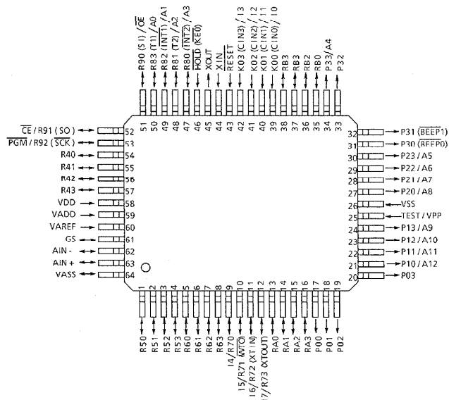
QFP64-P-1420-1.00A
