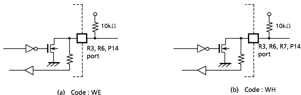
Figure 1-2. I/O code and external circuitry
