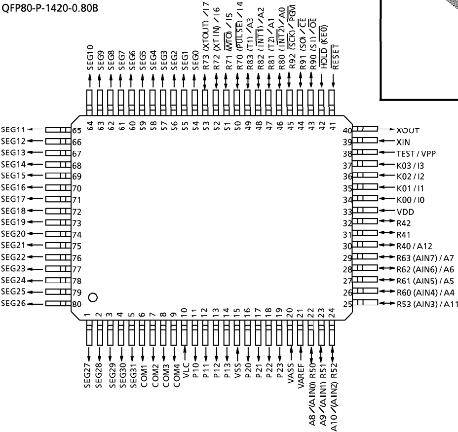
QFP80-P-1420-0.80B
