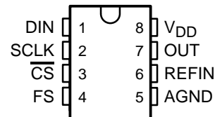
D OR DGK PACKAGE (TOP VIEW)
