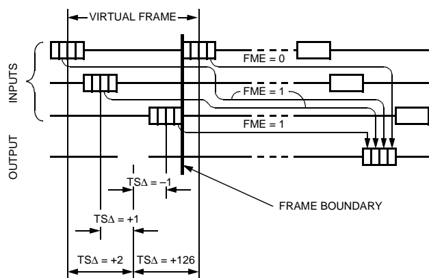
Figure 15. Constant Delay/Minimum Delay Example
