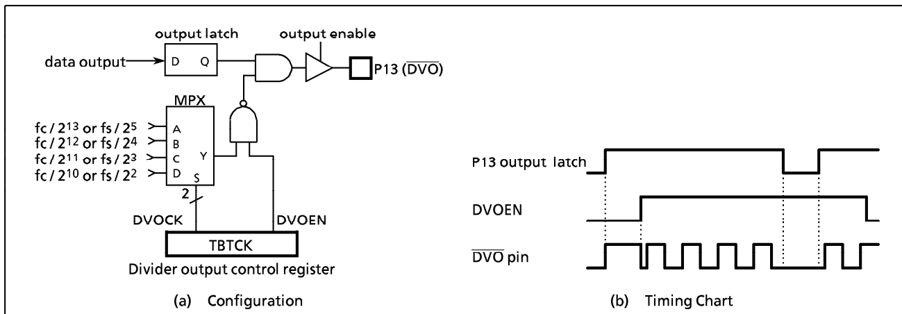
Figure 2-13. Divider Output
