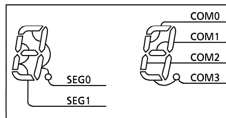
Figure 2-49. Example of COM, SEG Pin Connection (1/4 Duty)
