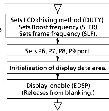
Figure 2-48. Initial Setting of LCD Driver
