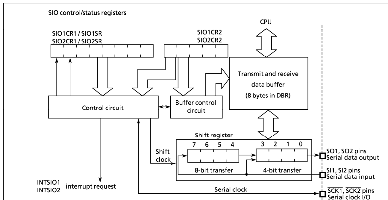
Figure 2-33. Serial Interfaces
