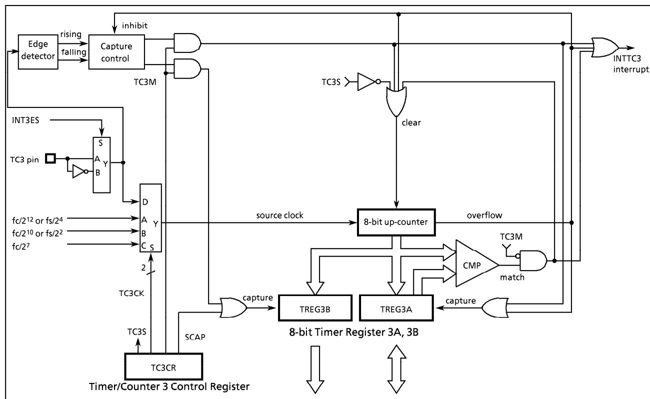
Figure 2-26. Timer/Counter 3
