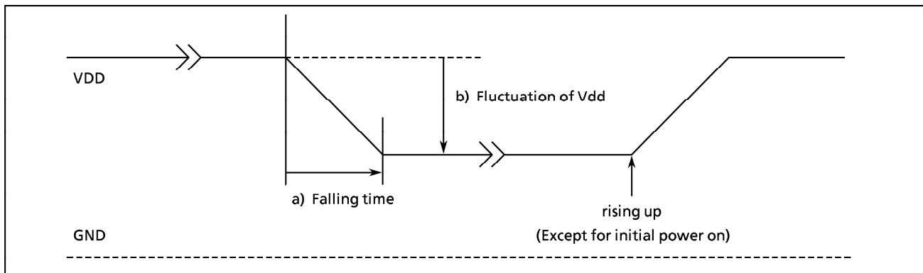
Fig. a The diagram for the falling time of Vdd
