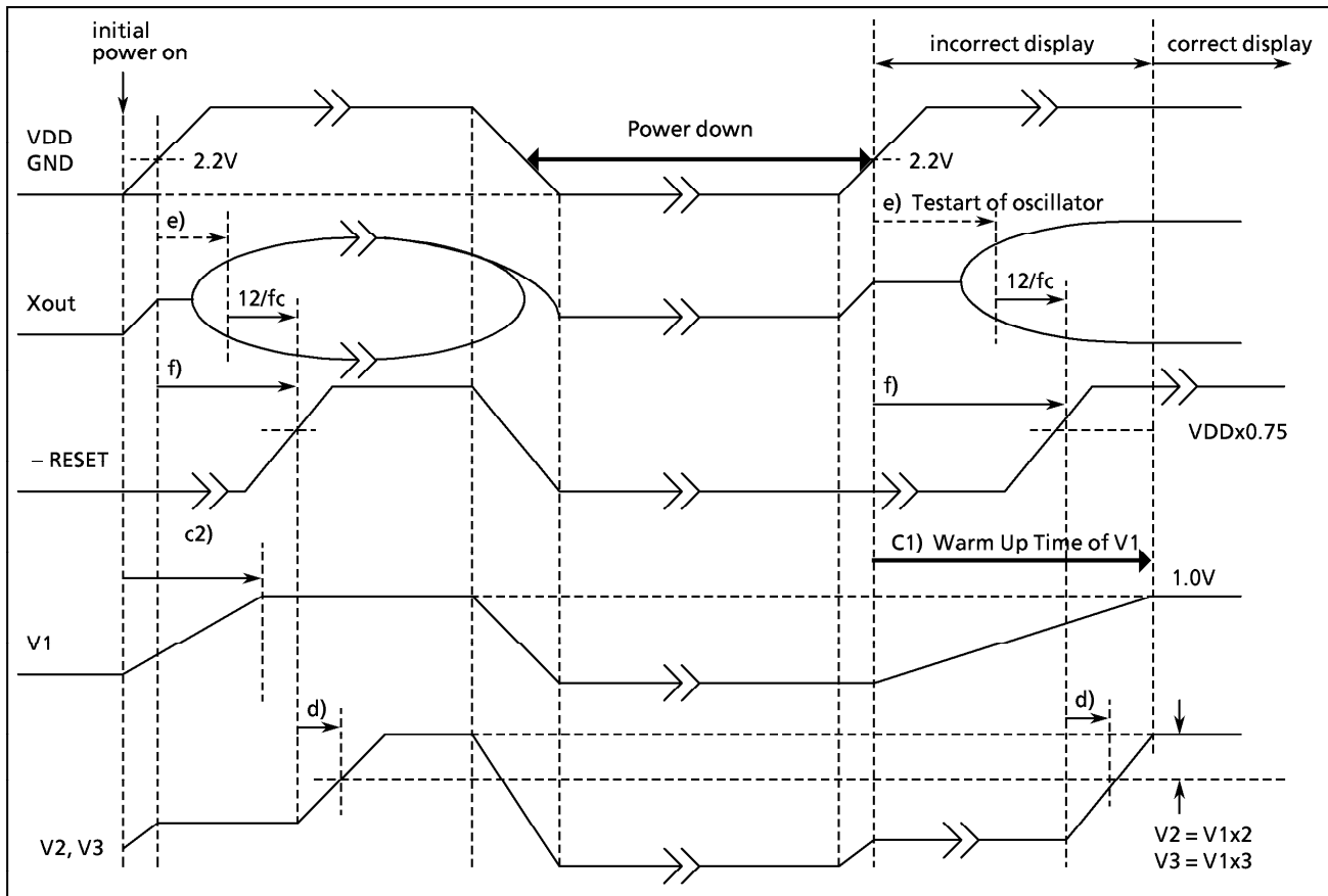
Fig. b The diagram for the warm up time of LCD Driver
