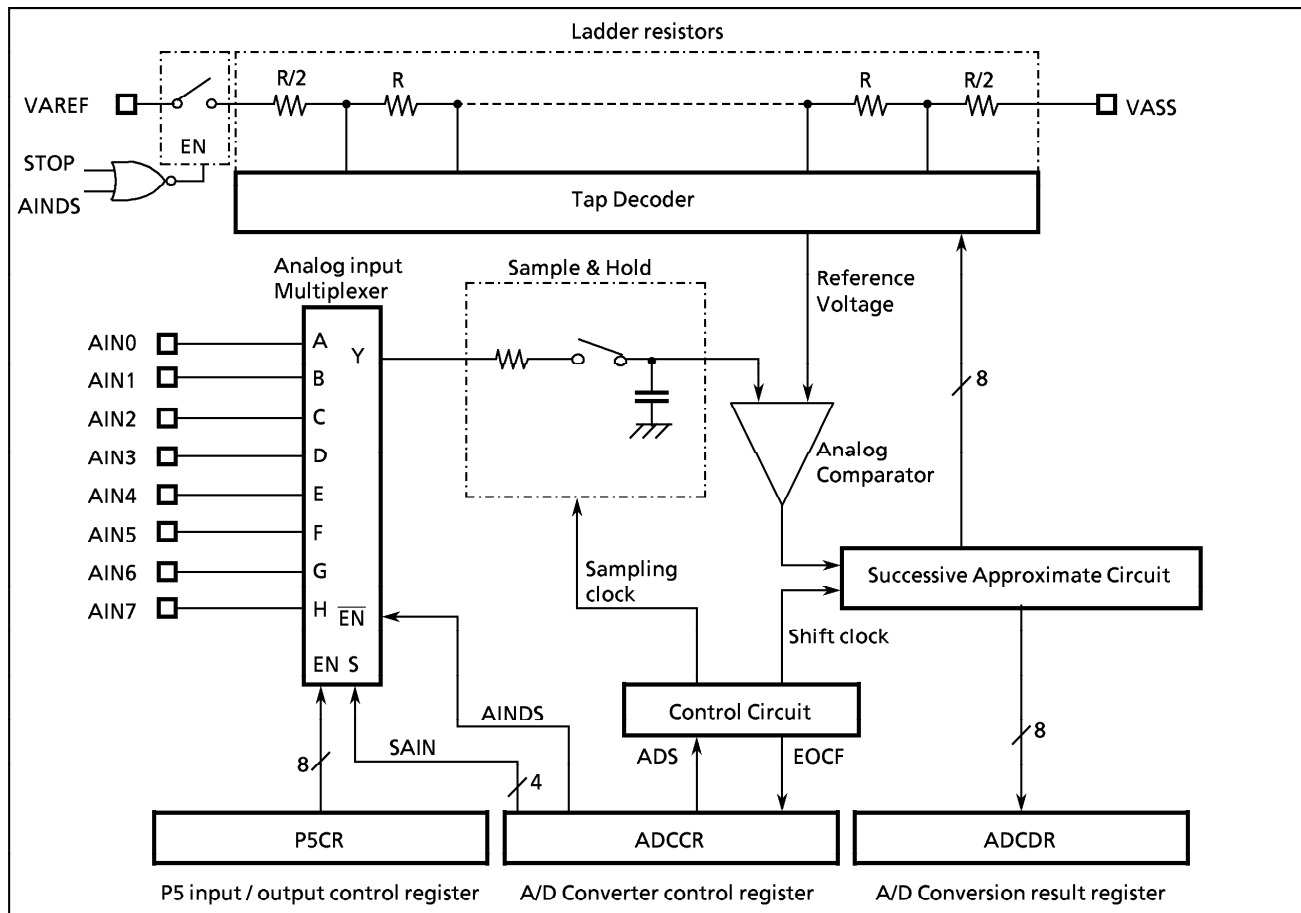
Figure 2-55. A/D Converter
