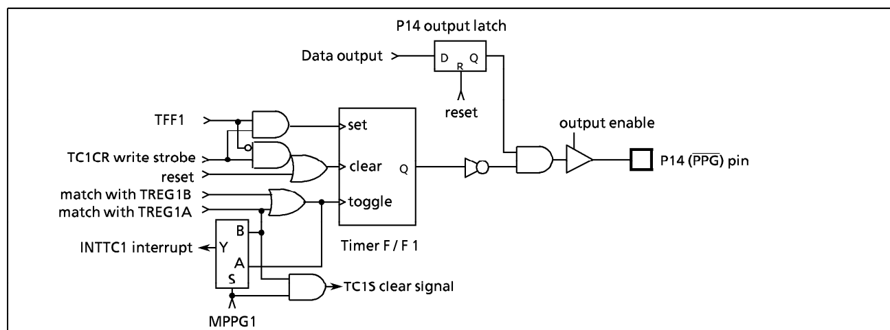
Figure 2-22. PPG Output
