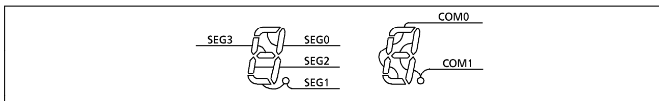
Figure 2-50. Example of COM, SEG Pin Connection
