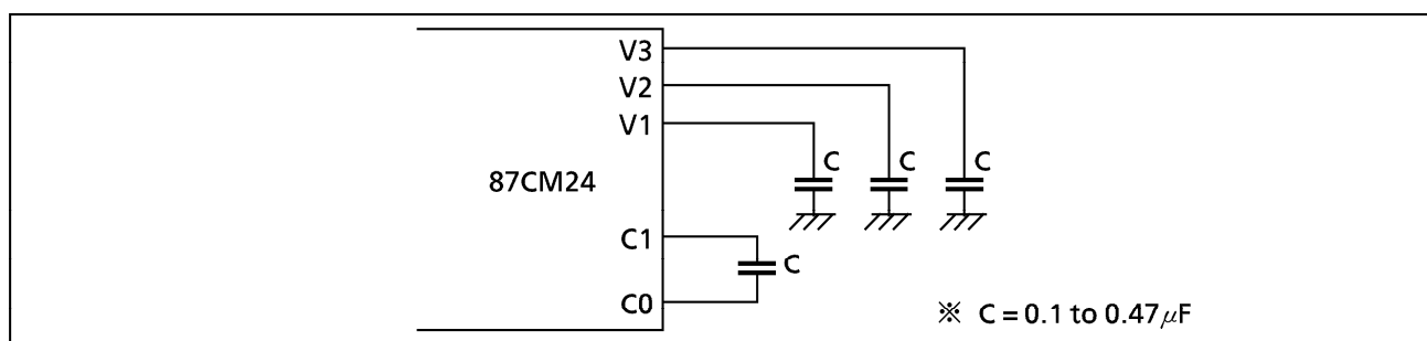
Figure 2-46. Example of a Booster Circuit
