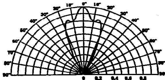
RADIATION PATTERN T_a = 25^\circ\text{C}
