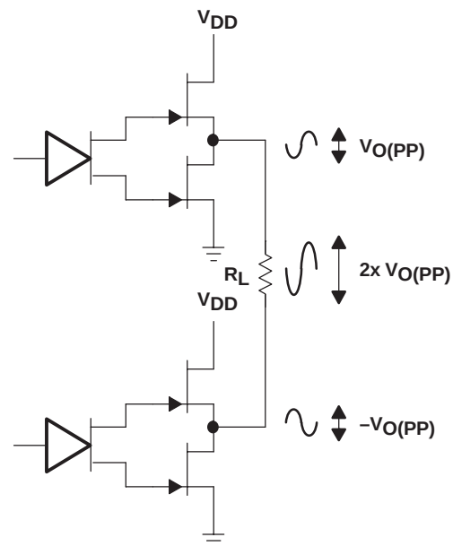
Figure 31. Differential Output Configuration
