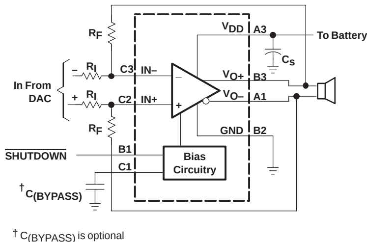
Figure 28. Typical Differential Input Application Schematic
