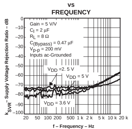
SUPPLY VOLTAGE REJECTION RATIO
