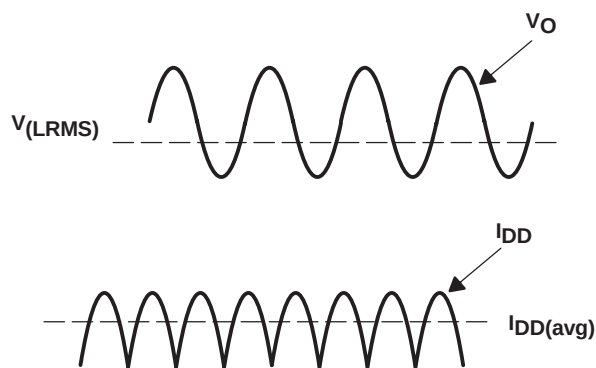
Figure 33. Voltage and Current Waveforms for BTL Amplifiers
