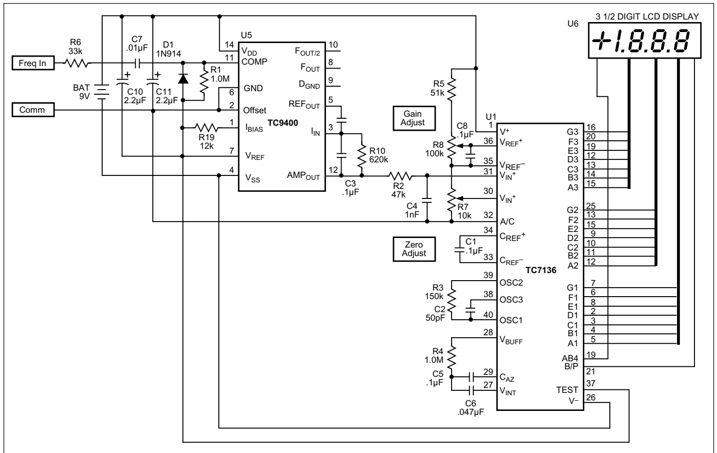
FIGURE 3: Schematic: battery powered frequency meter (0 to 20kHz).
