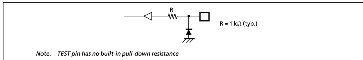
Figure 1-2. TEST Pin
