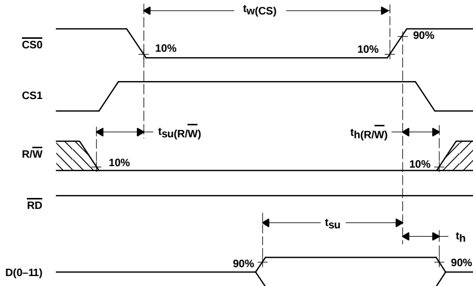
Figure 37. Write Timing Diagram Using \overline{R/W} ( \overline{CS0} -controlled)
