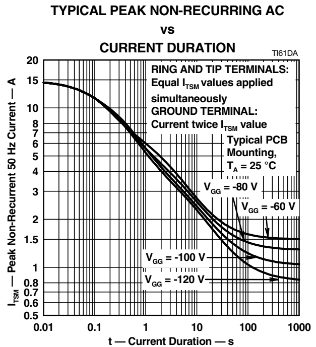
Figure 3. TYPICAL NON-REPETITIVE PEAK ON- STATE CURRENT AGAINST DURATION
