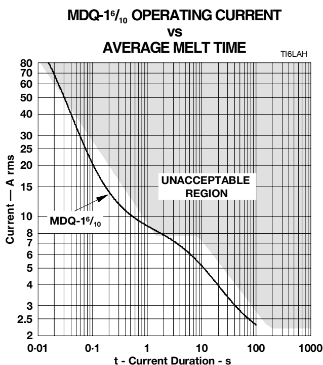
Figure 17. MDQ-1 6 / 10 CURRENT-TIME
