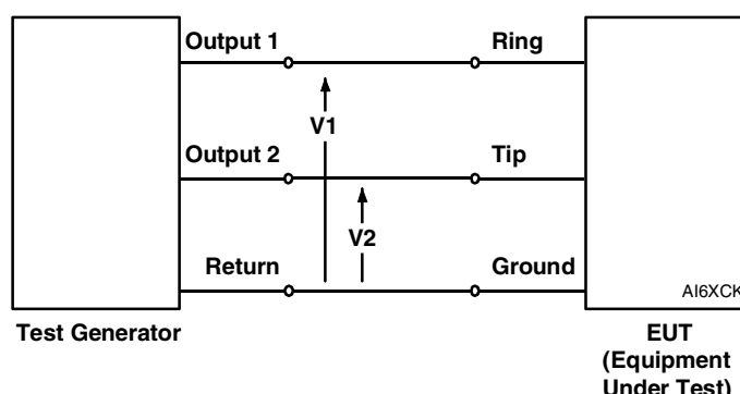
Figure 14. LONGTITUDINAL (ALSO CALLED COMMON MODE) TESTING
