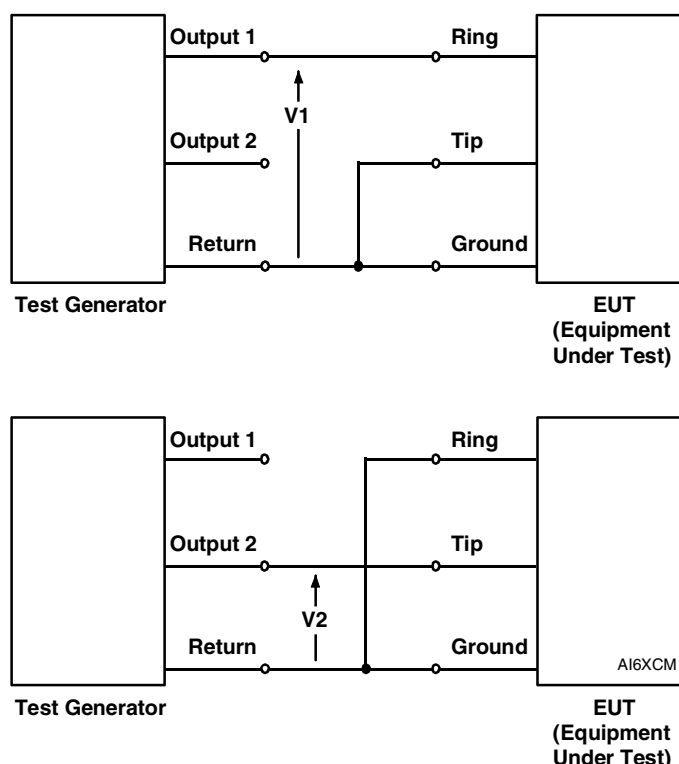
Figure 15. TRANSVERSE (ALSO CALLED DIFFERENTIAL OR METALLIC) TESTING
