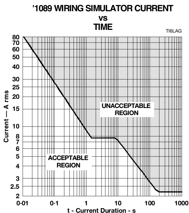
Figure 16. WIRING SIMULATOR CURRENT-TIME
