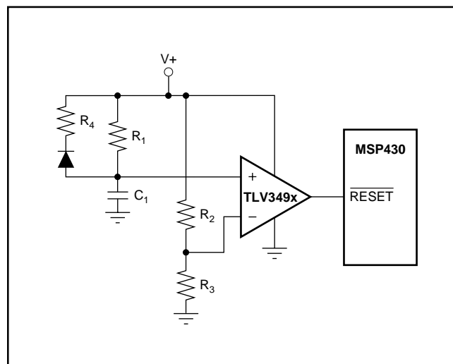
FIGURE 4. The TLV349x Configured as a Reset Circuit for the MSP430.
