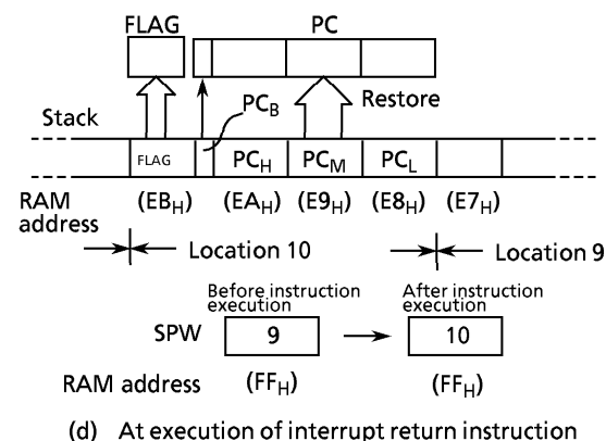
Figure 2-7. Stack Access (Save/Restore)
