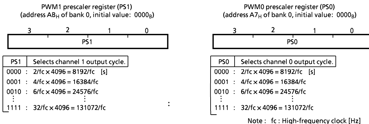
Figure 3-34. PWM Prescaler Register
