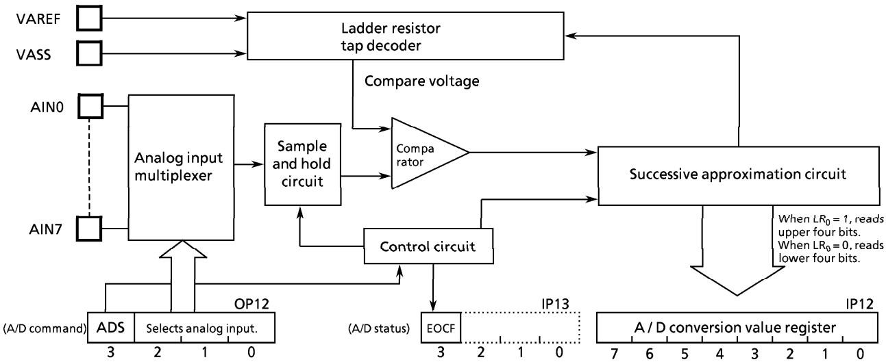
Figure 3-27. Configuration of A/D Converter
