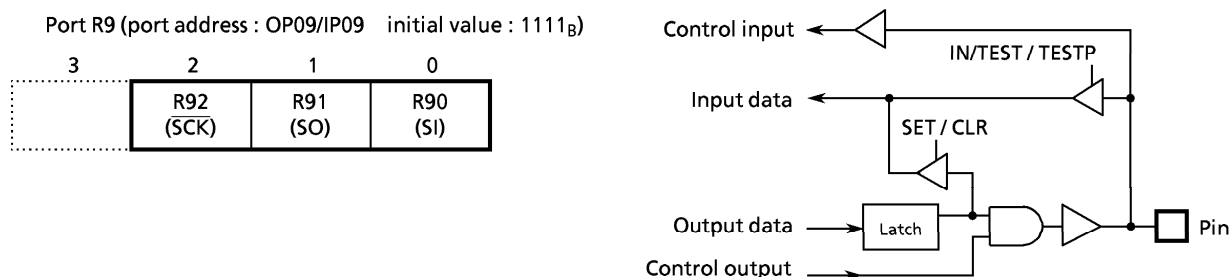
Figure 3-6. Port R9
