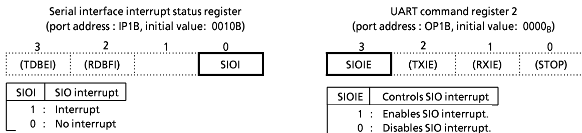
Figure 3-45. Serial Interface Interrupt Status Register and UART Command Register 2
