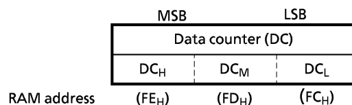
Figure 2-8. Data Counter
