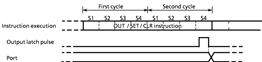
Figure 3-2. Output Timing
