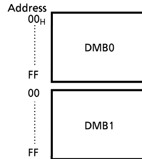
Figure 2-11. Data Memory (RAM)
