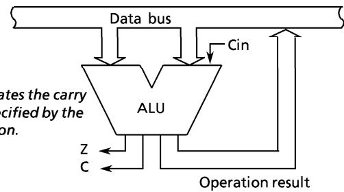
Figure 2-12. ALU
