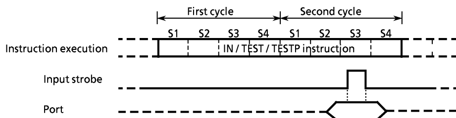
Figure 3-1. Input Timing
