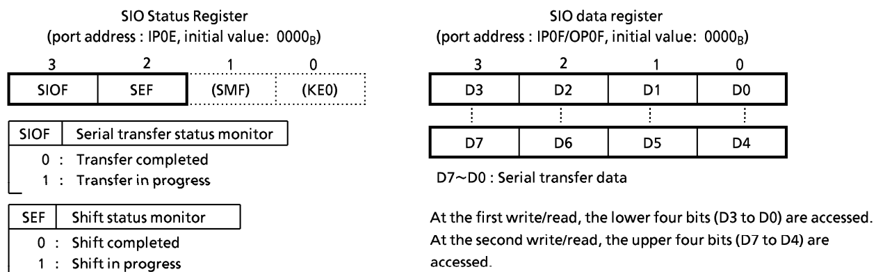
Figure 3-43. SIO Status Register and SIO Data Register
