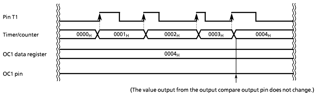
Figure 3-21 (c). Event Count Interrupt Usage Example (output compare channel: OC1) (Event input pin: T1 (counts at the rising edge of input waveform (CPSEL = 101 B ))
