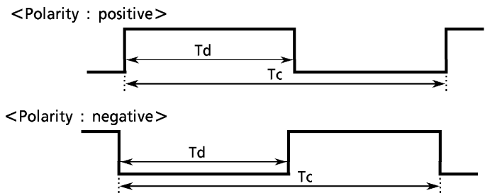
Figure 3-36. PWM Output Waveform
