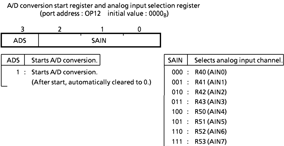
Figure 3-28. A/D Conversion Start Register and Analog Input Selection Register
