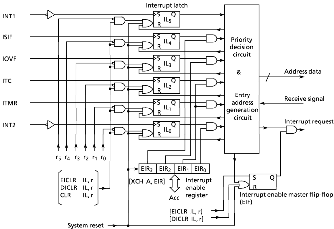
Figure 2-24. Interrupt Control Circuit Block Diagram
