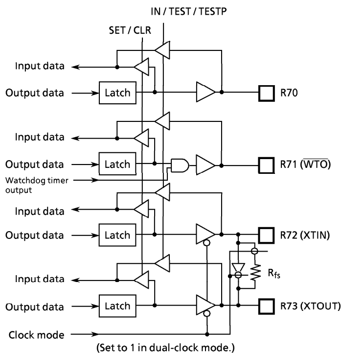
Figure 3-4 (c). Port R7
