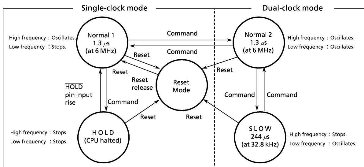
Figure 2-18. Operating Mode Transition Diagram
