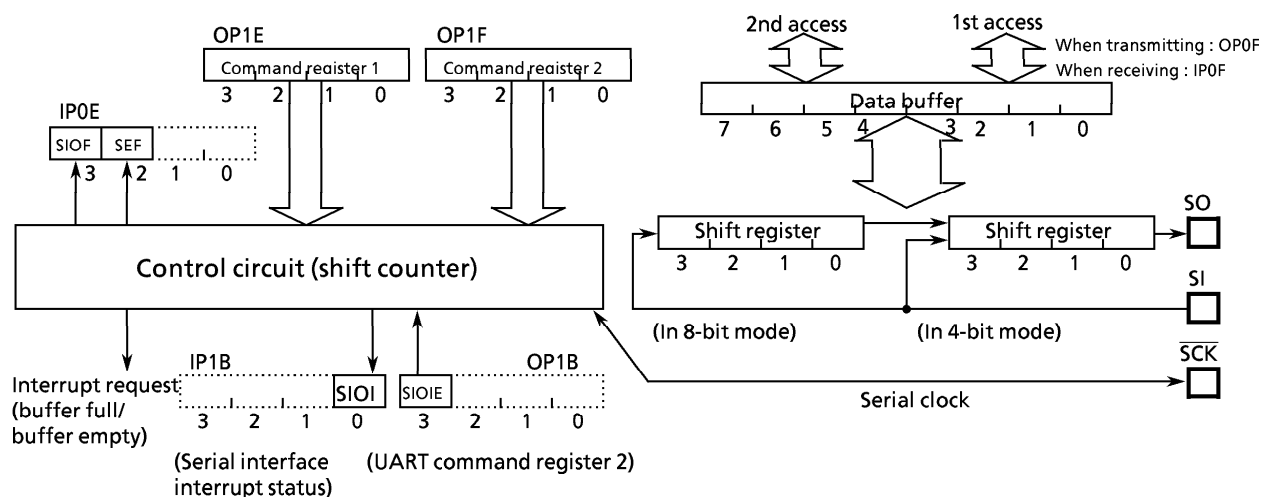
Figure 3-42. Configuration of Synchronous Serial Interface
