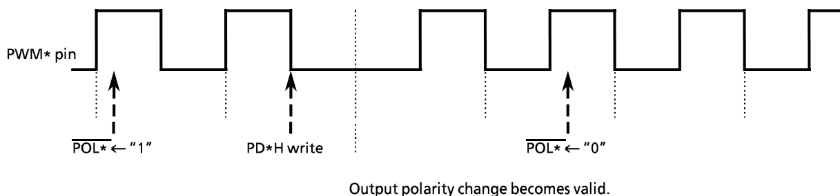
Figure 3-41. Output Polarity Change
