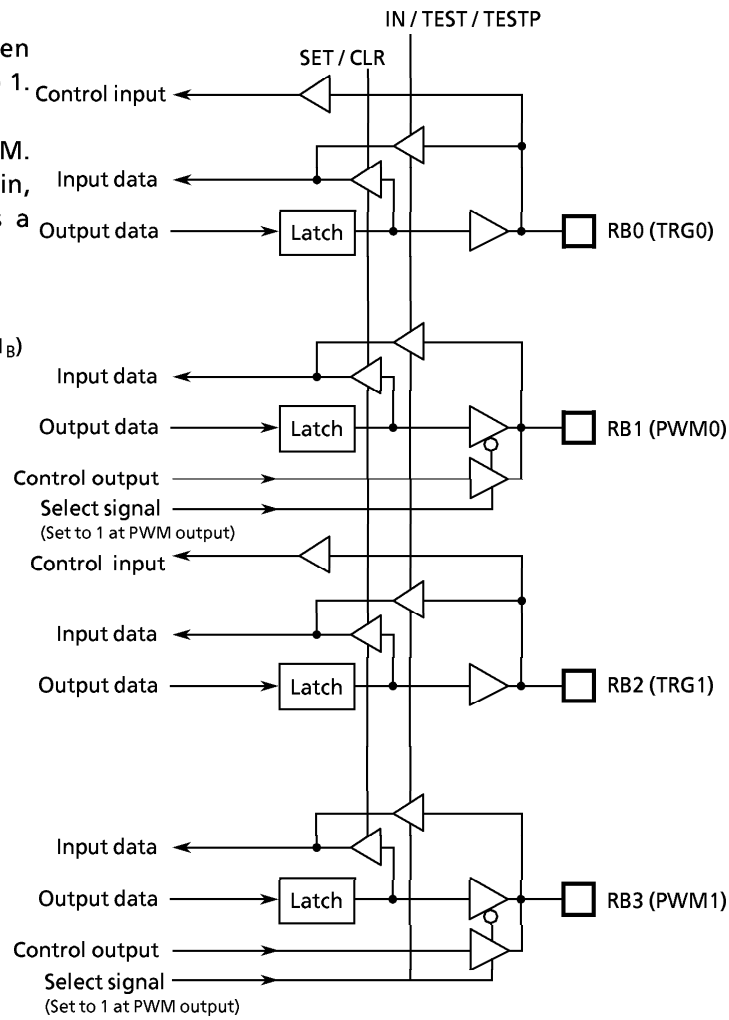
Figure 3-8. Port RB
