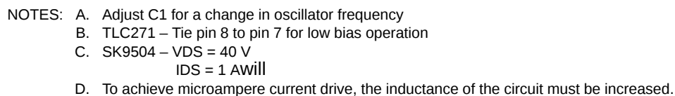
Figure 28. Micropower Switching Regulator
