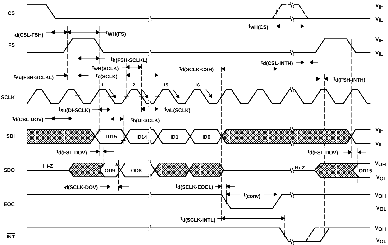
Figure 16. Critical Timing (Normal Sampling, FS is Active)
