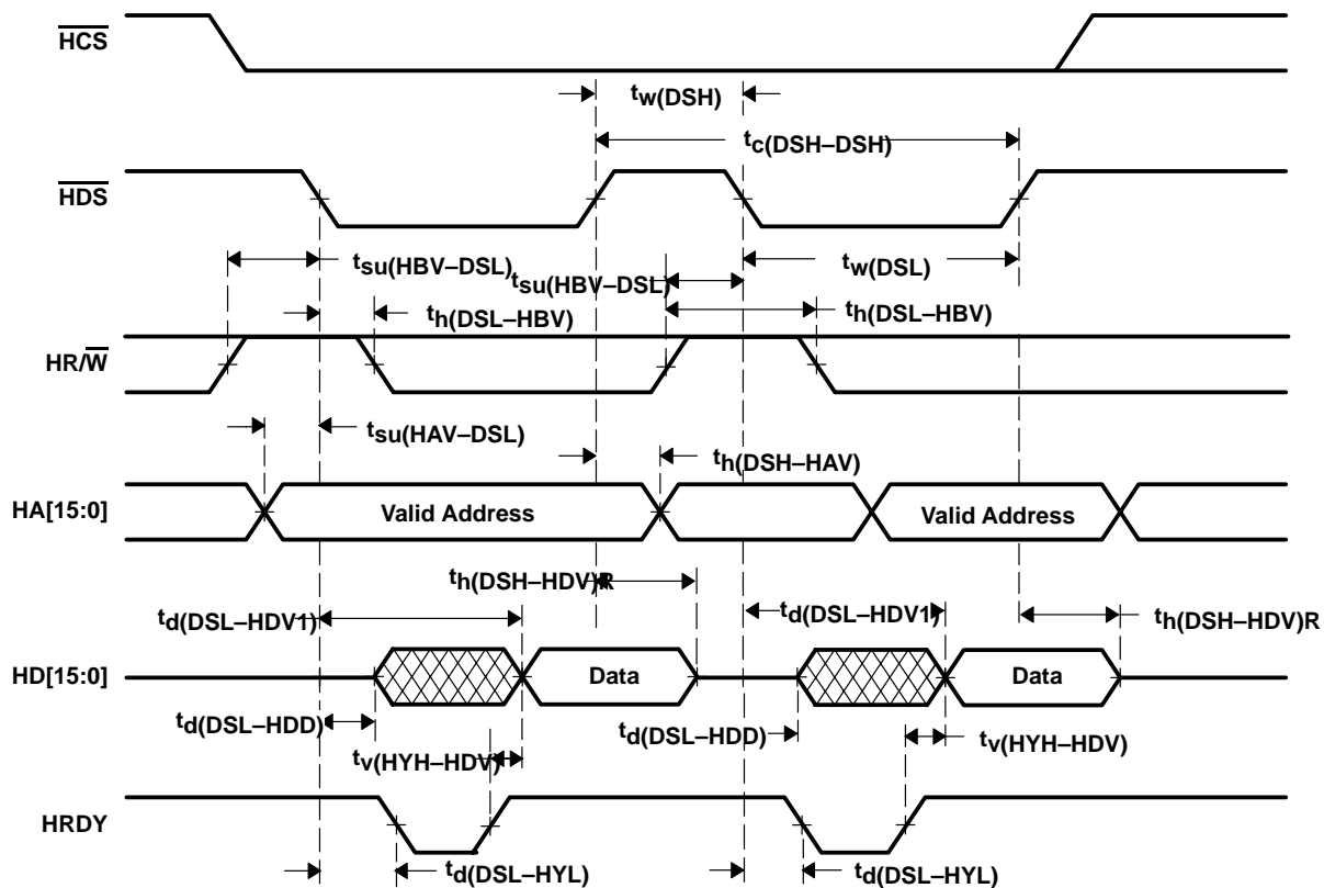
Figure 5–32. HPI-16 Mode, Nonmultiplexed Read Timings
