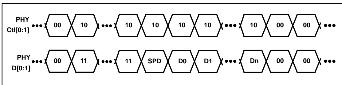
Figure 6–5. Receive Timing
