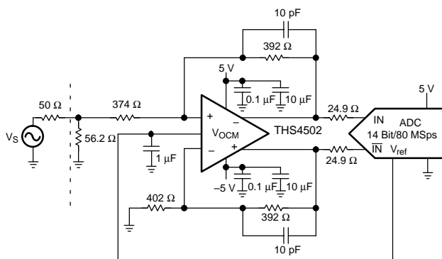
APPLICATION CIRCUIT DIAGRAM
