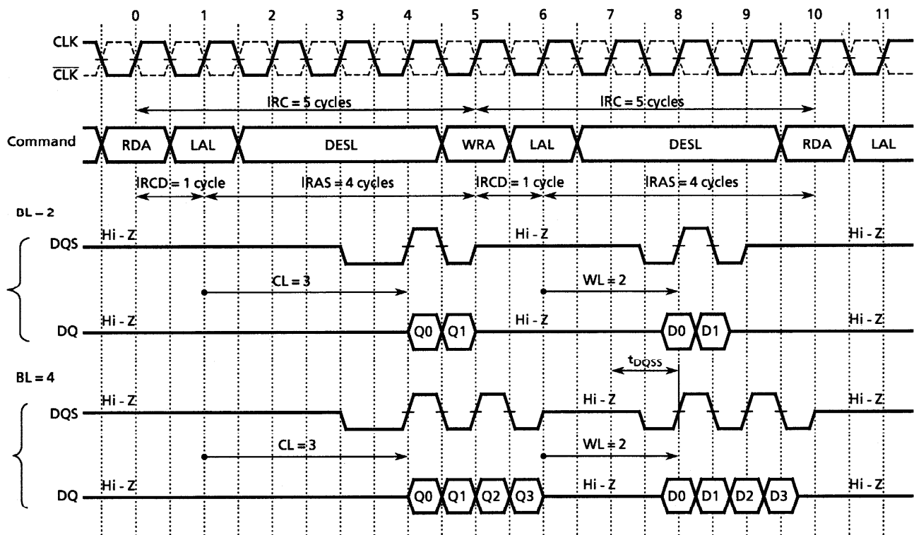
Single Bank Read-Write Timing (CL=3)
