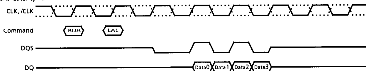
Addressing sequence for Sequential mode
