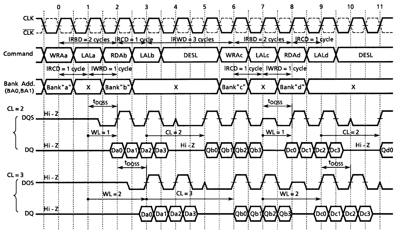
Multiple Bank Read-Write Timing (BL=4)
