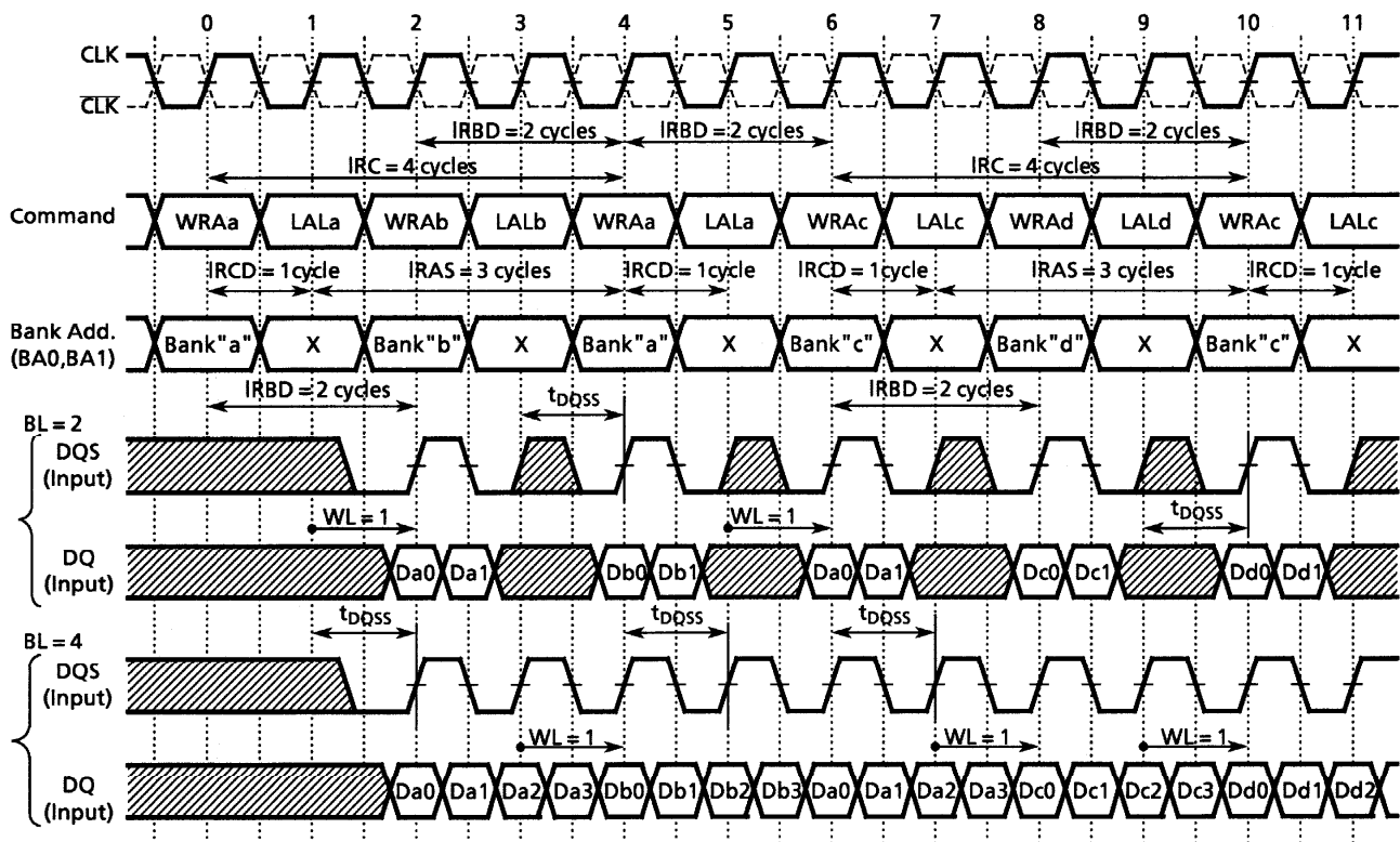
Multiple Bank Write Timing (CL=3)
