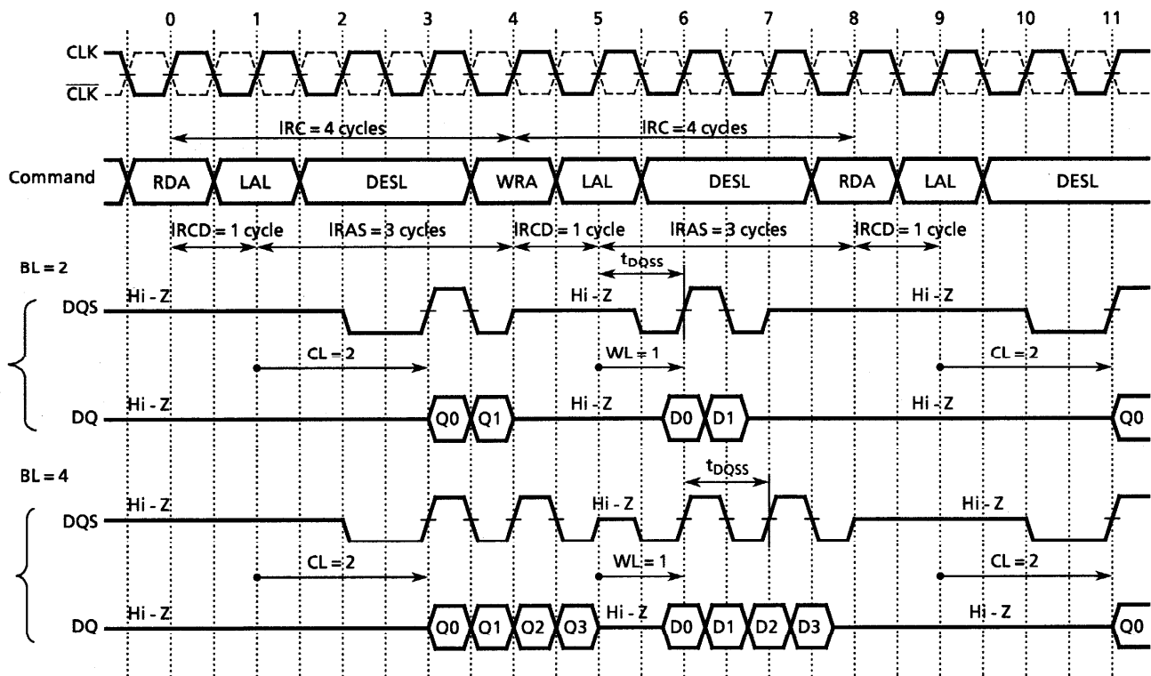
Single Bank Read-Write Timing (CL=2)
