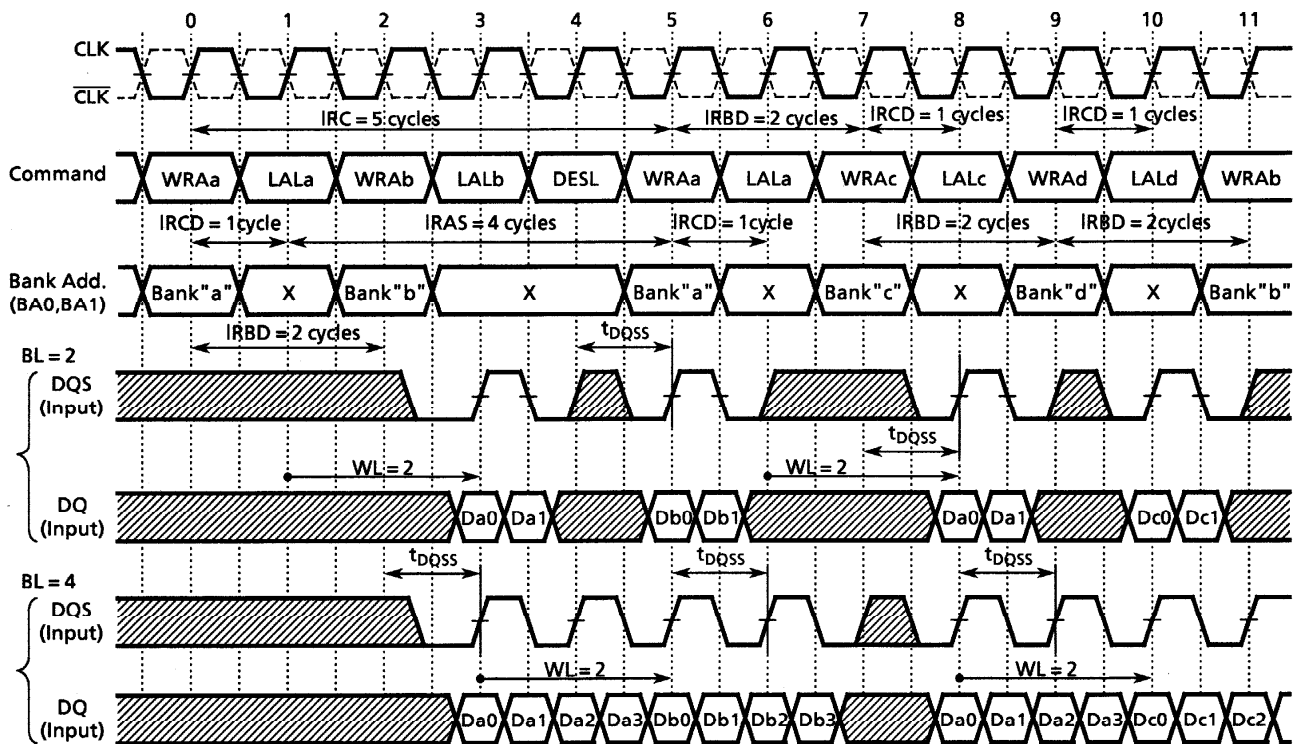
Multiple Bank Write Timing (CL=3)
