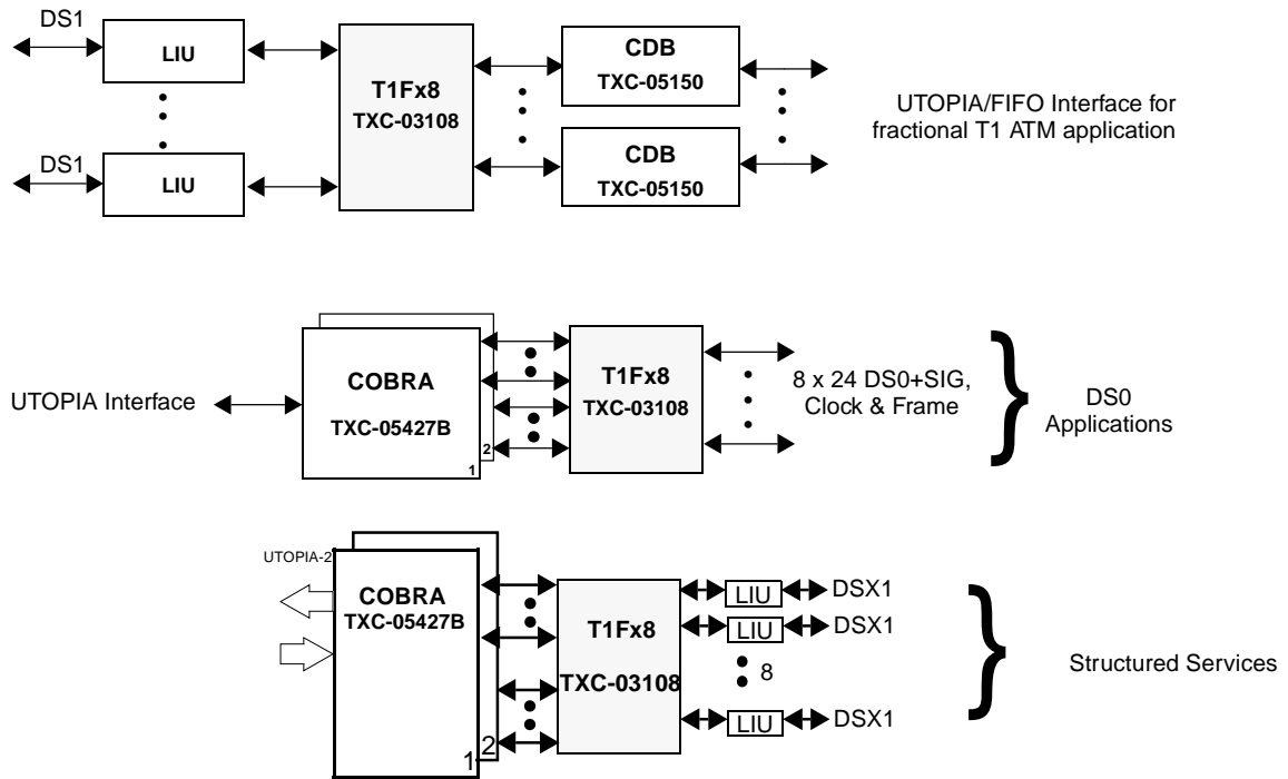
Figure 2. Example T1F x 8 TXC-03108 ATM Applications
