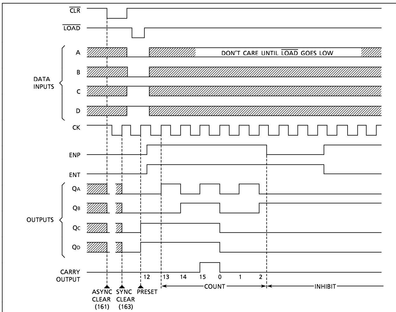
TIMING CHART
