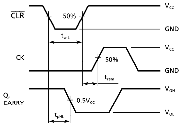
CLEAR MODE (TC74AC163) (Fig. 5)
