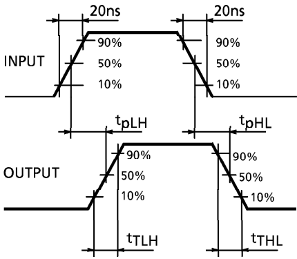
WAVEFORM
