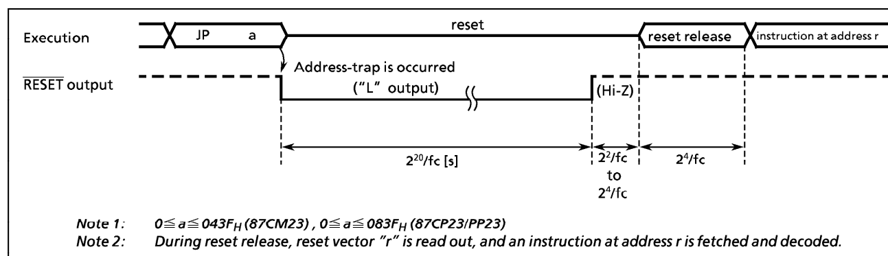
Figure 1-31. Address-Trap-Reset
