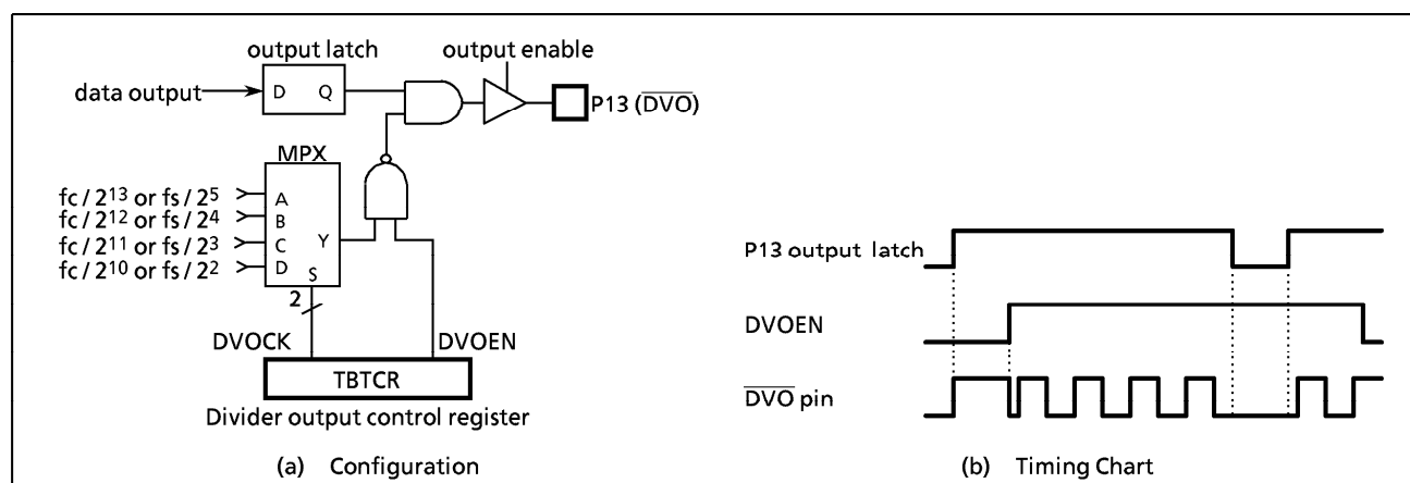
Figure 2-13. Divider Output
