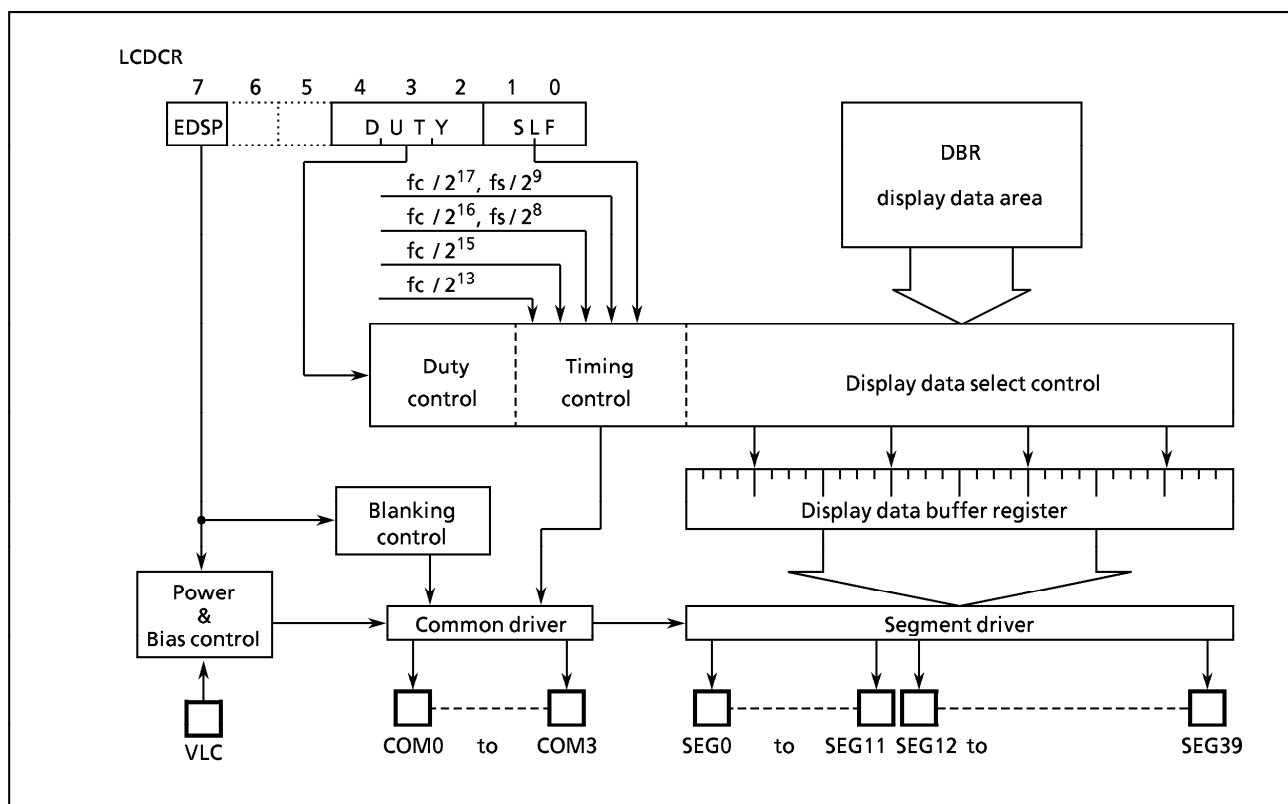
Figure 2-43. LCD driver
