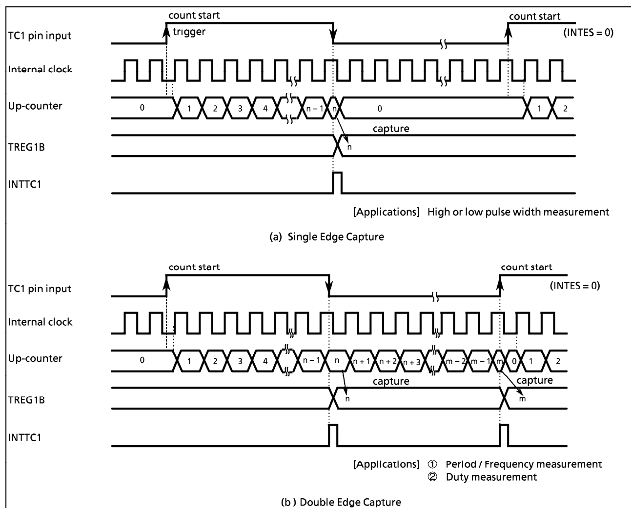
Figure 2-20. Pulse Width Measurement Mode Timing Chart
