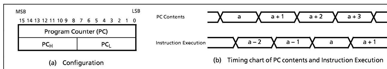
Figure 1-3. Program Counter
