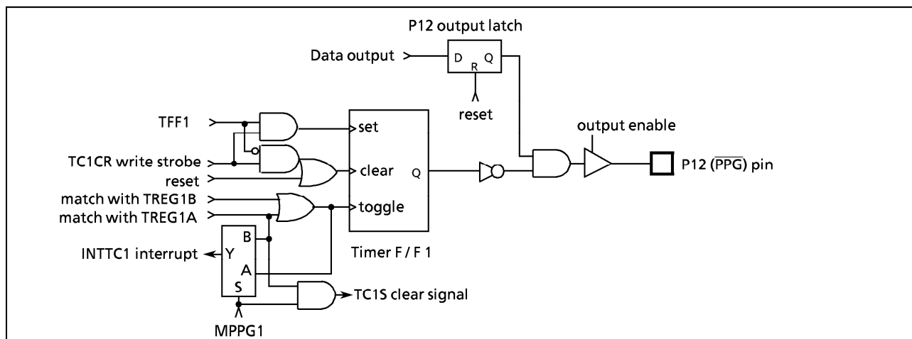
Figure 2-26. PPG Output
