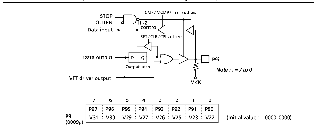
Figure 2-12. Port P9
