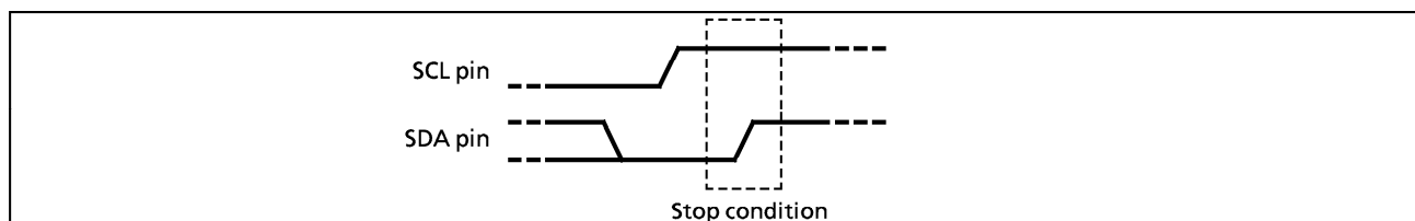
Figure 2-45. Stop Condition Generation
