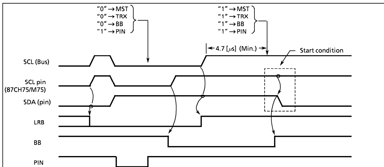
Figure 2-53. Timing Diagram when Restarting the 87CH75/M75
