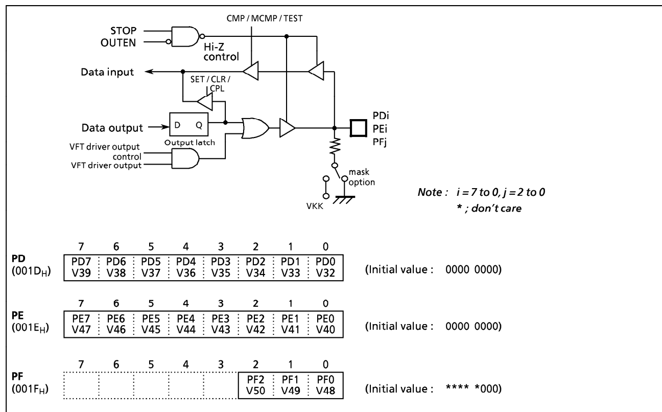
Figure 2-13. PD, PE, PF Ports
