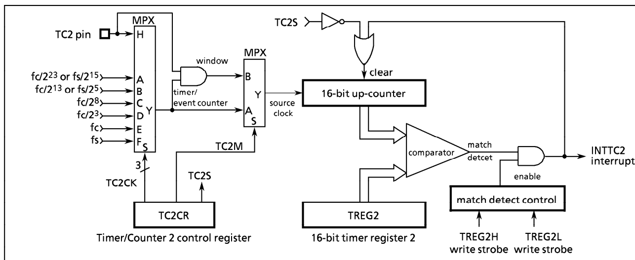
Figure 2-27. Timer/Counter 2 (TC2)
