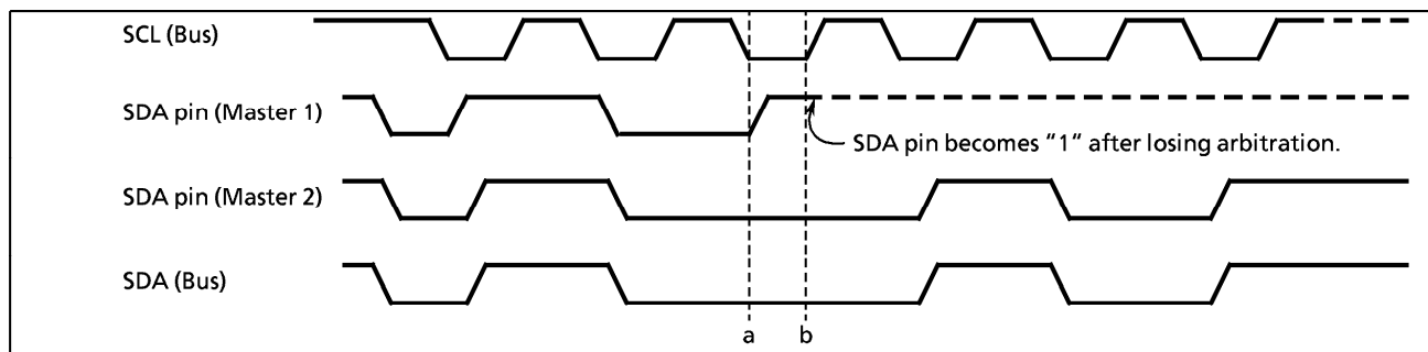
Figure 2-46. Arbitration Lost
