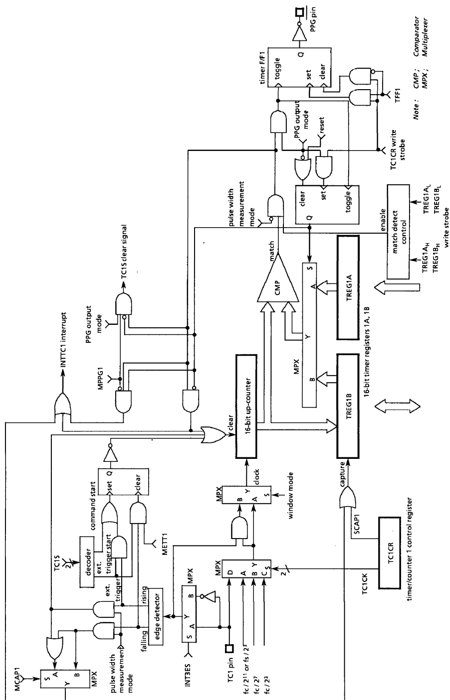
Figure 2-18. Timer/Counter 1
