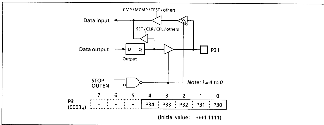
Figure 2-5. Port P3
