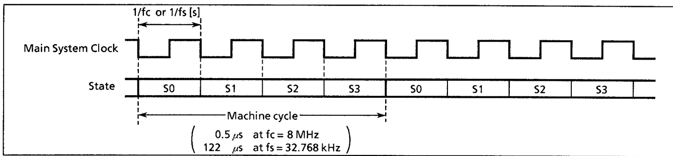
Figure 1-13. Machine Cycle
