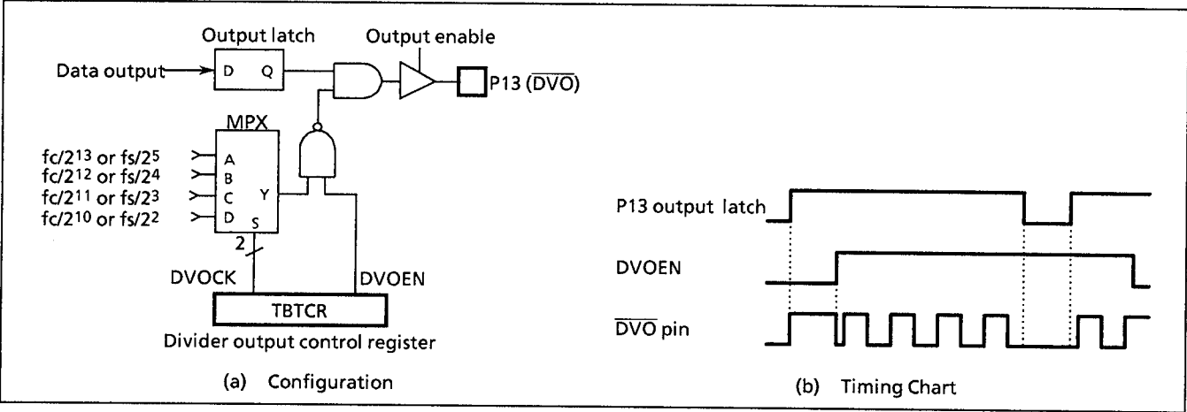
Figure 2-12. Divider Output
