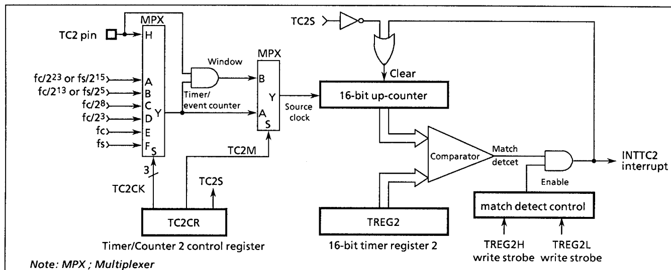
Figure 2-22. Timer/Counter 2 (TC2)
