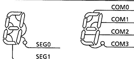
Figure 2-52. Example of COM, SEG Pin Connection (1/4 Duty)
