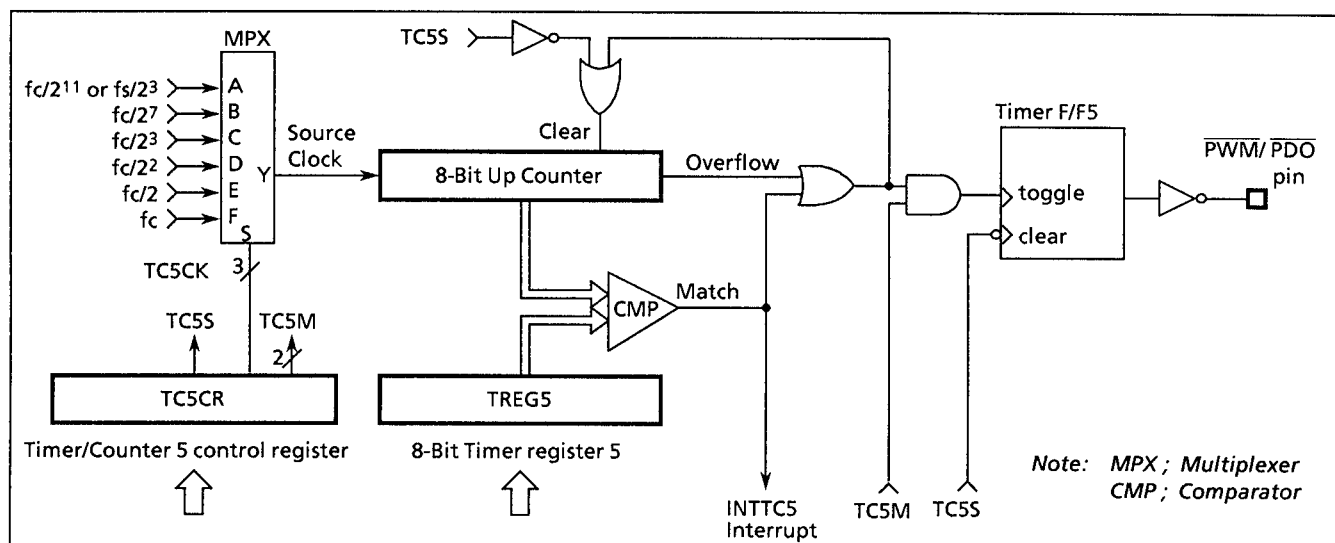
Figure 2-28. Timer/Counter 5 (TC5)
