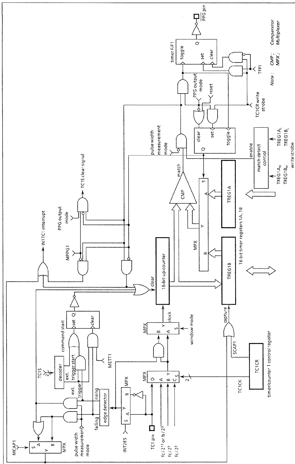
Figure 2-14. Timer/Counter 1
