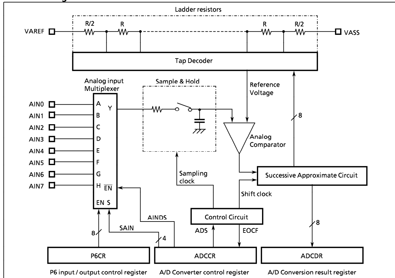
Figure 2-43. A/D Converter
