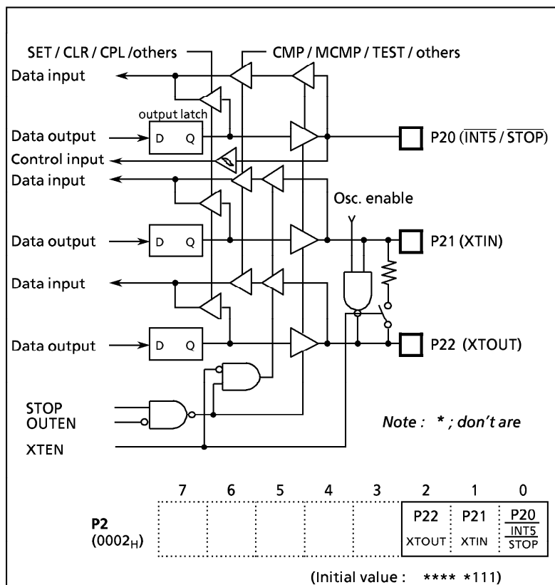
Figure 2-5. Port P2
