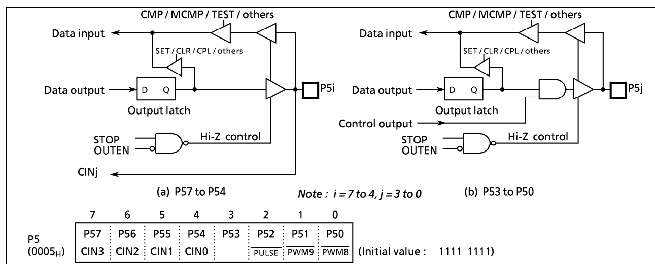
Figure 2-6. Ports P5
