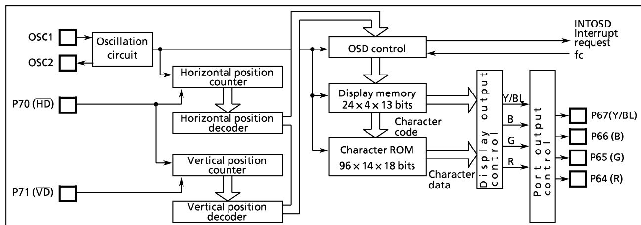
Figure 2-35. OSD Circuit
