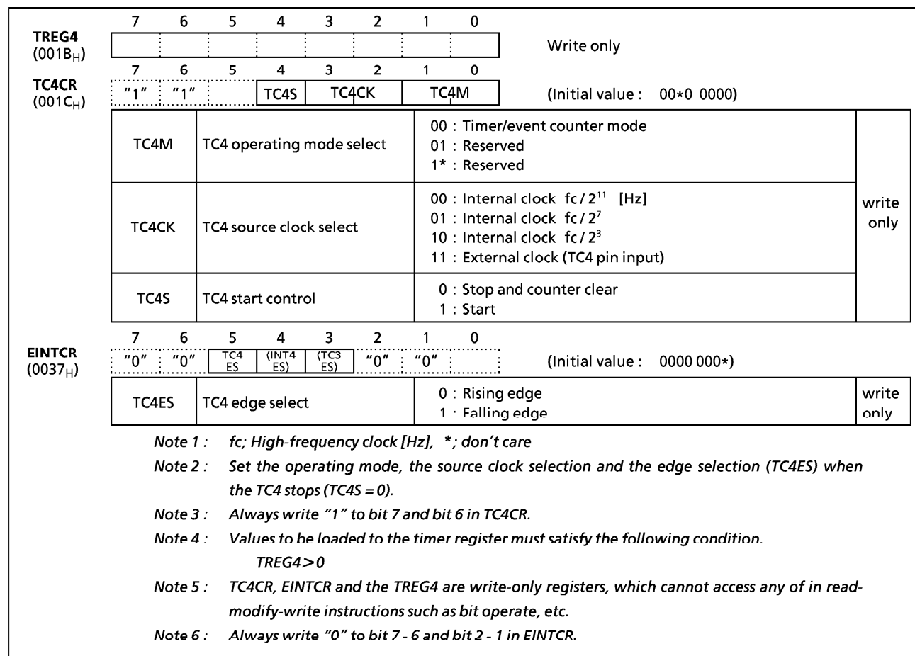
Figure 2-20. Timer Register 4 and TC4 Control Registers
