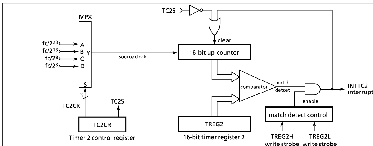
Figure 2-14. Timer 2 (TC2)
