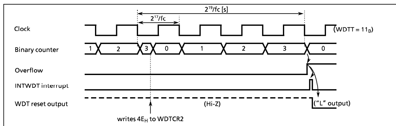
Figure 1-28. Watchdog Timer Interrupt / Reset
