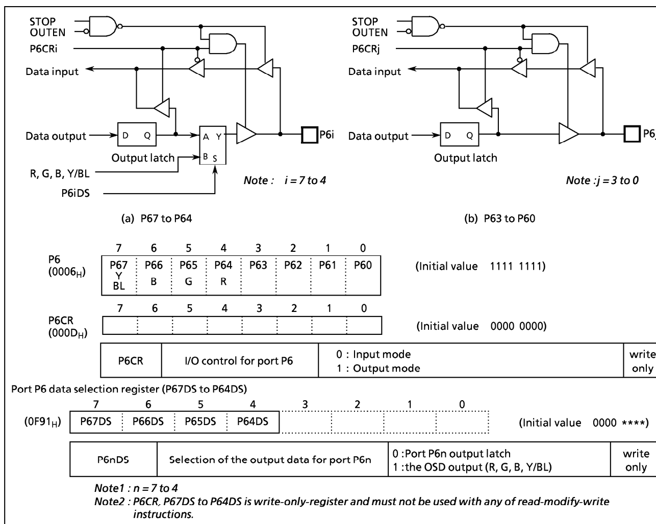
Figure 2-7. Ports P6, P6CR, and P67DS to P64DS
