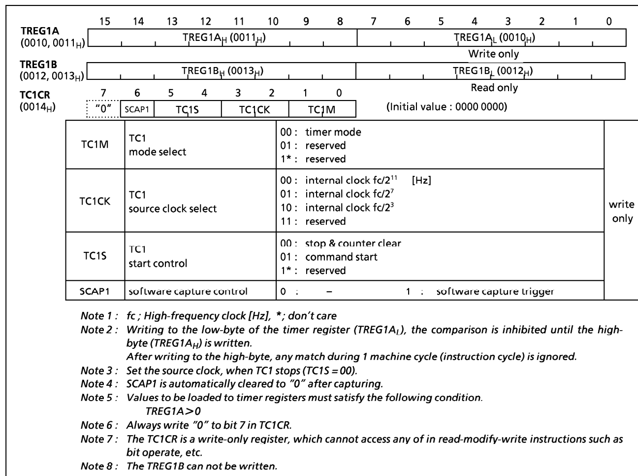
Figure 2-12. Timer Registers and TC1 Control Register
