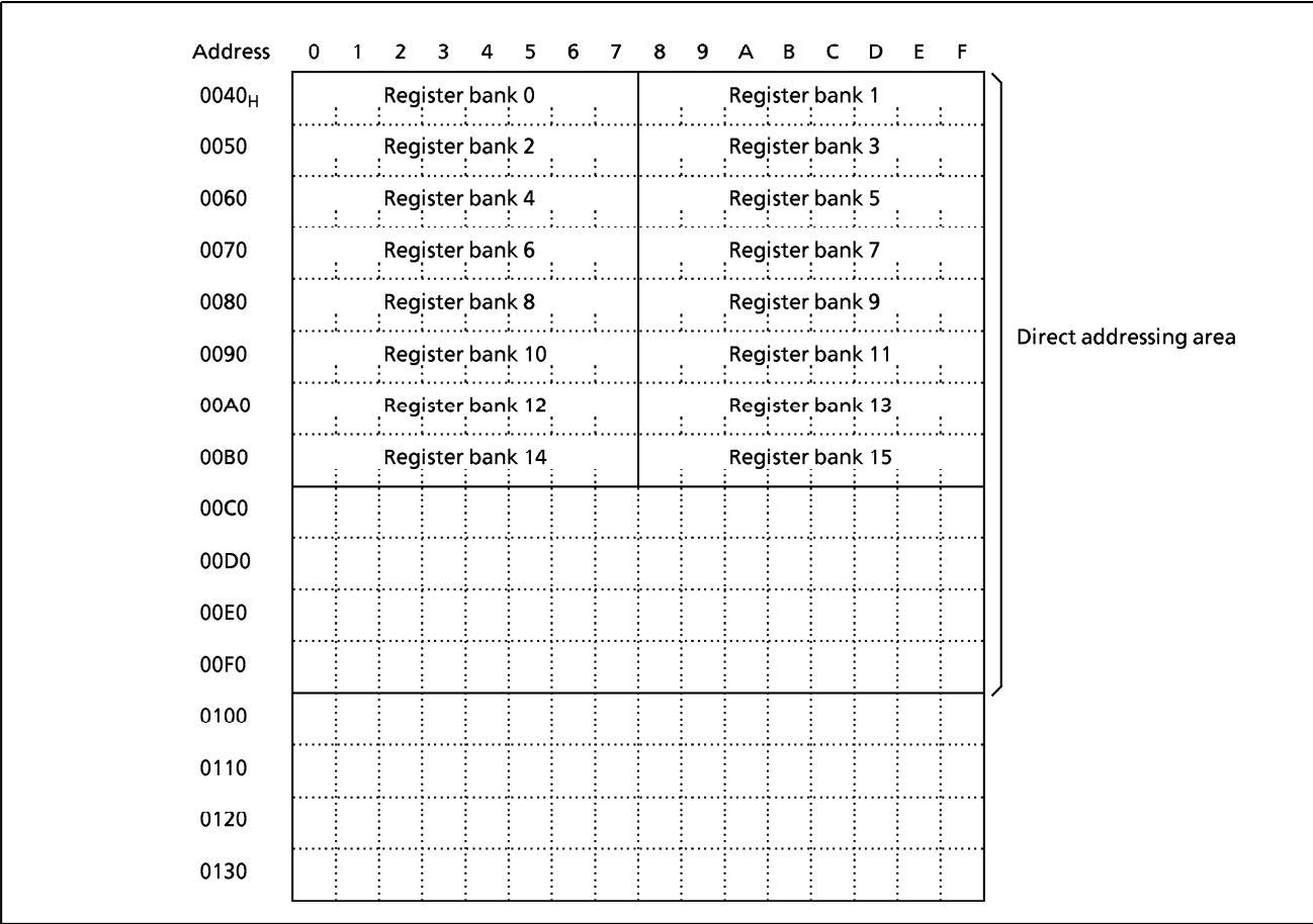
Figure 1-5. Data Memory Map
