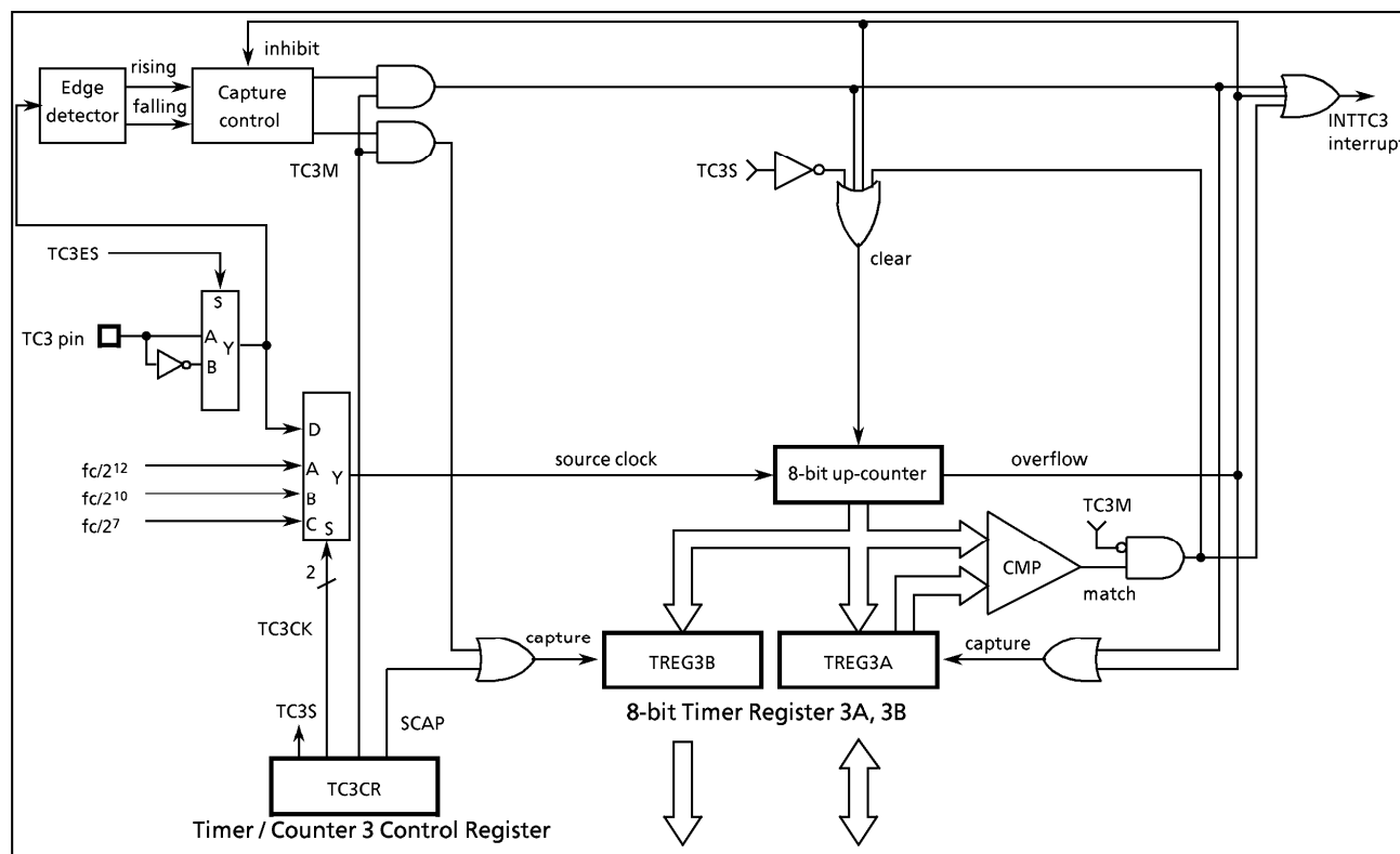
Figure 2-16. Timer/Counter 3
