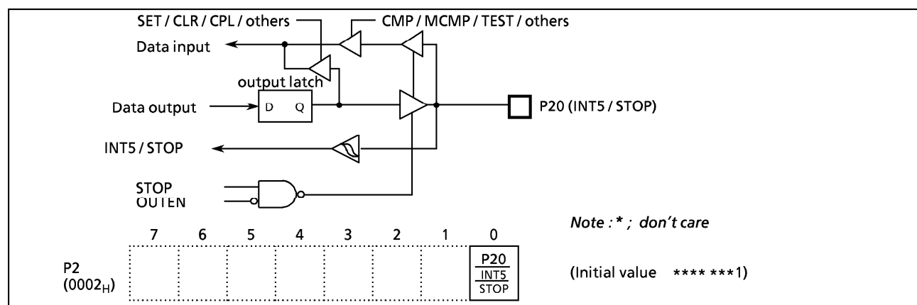
Figure 2-3. Port P2
