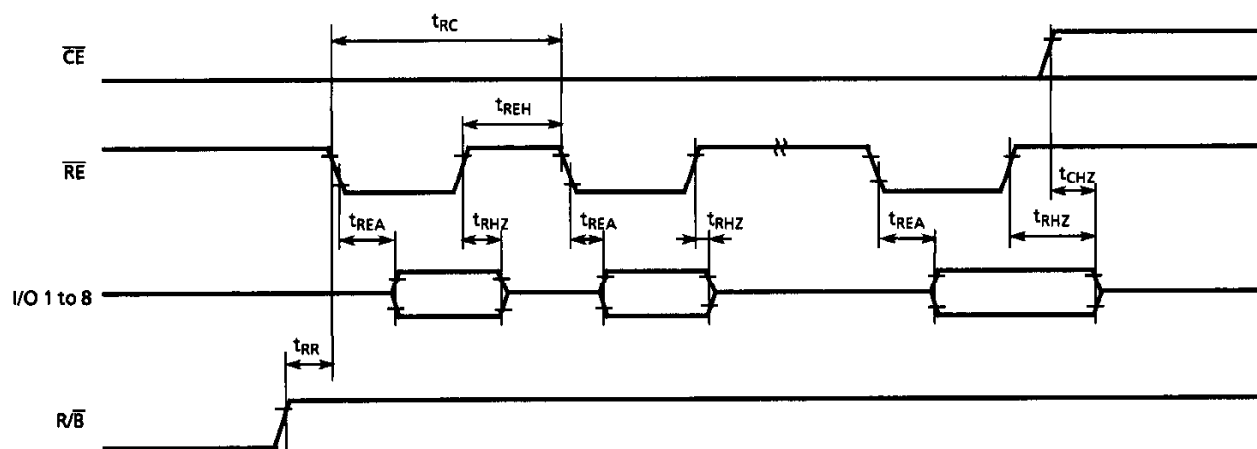
Serial Read Cycle Timing Diagram
