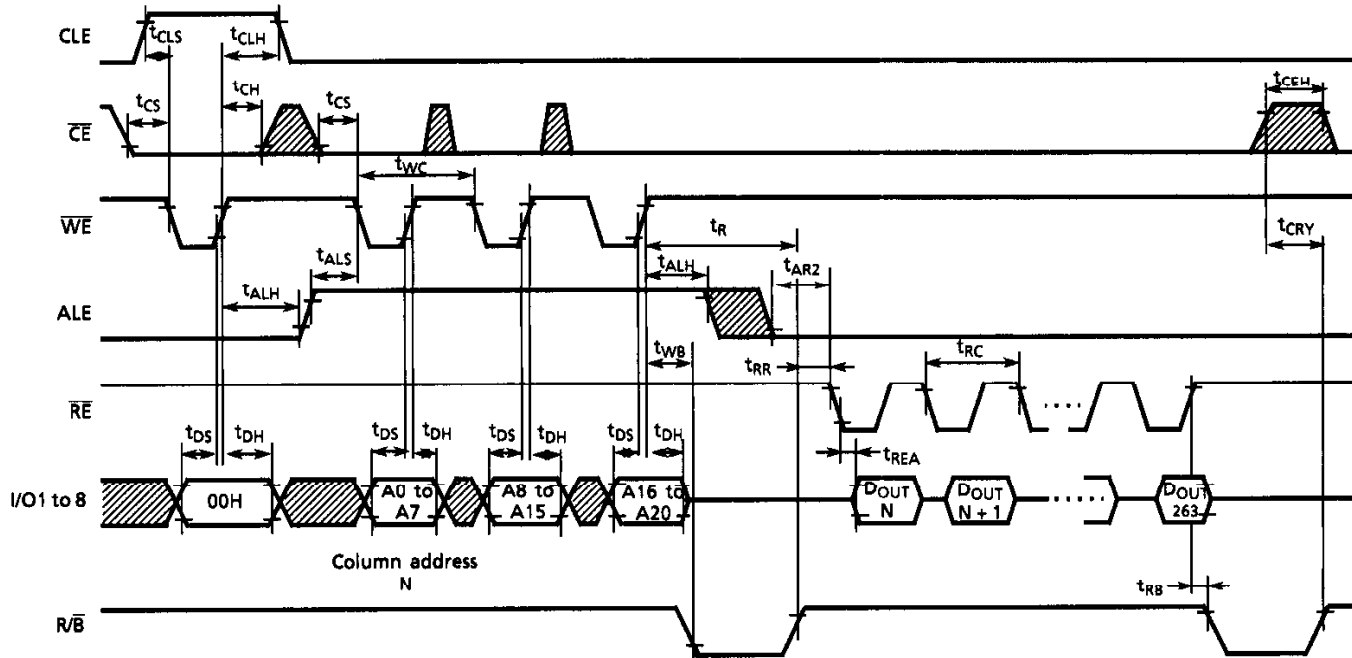
Read Cycle (1) Timing Diagram
