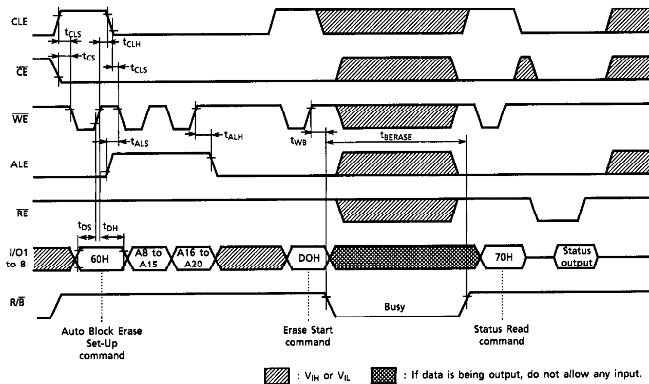
Auto Block Erase Timing Diagram
