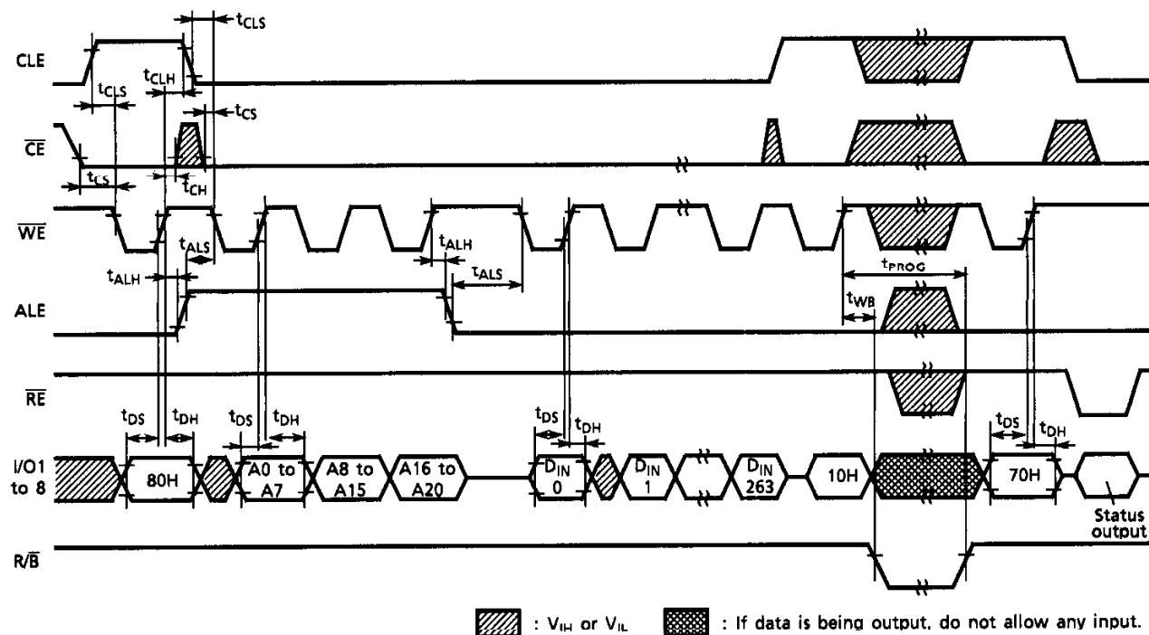
Auto Program Operation Timing Diagram
