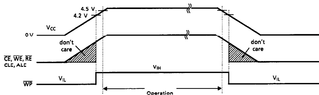
Figure 29. TC5816 Power On/Off Sequence
