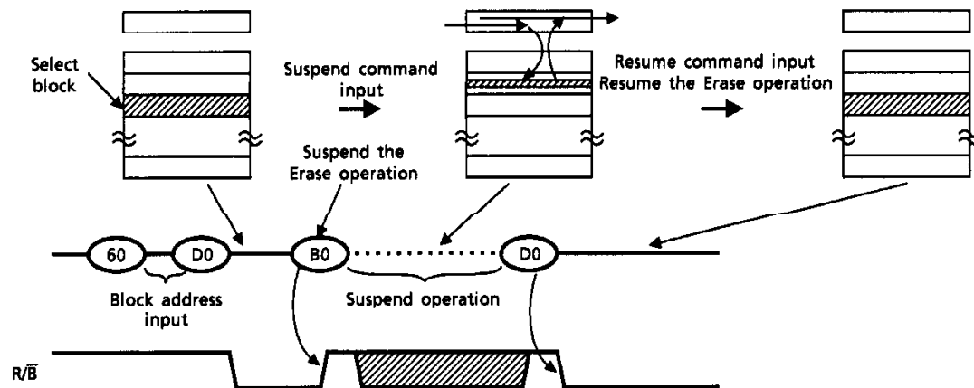
Figure 9. Suspend/Resume Operation
