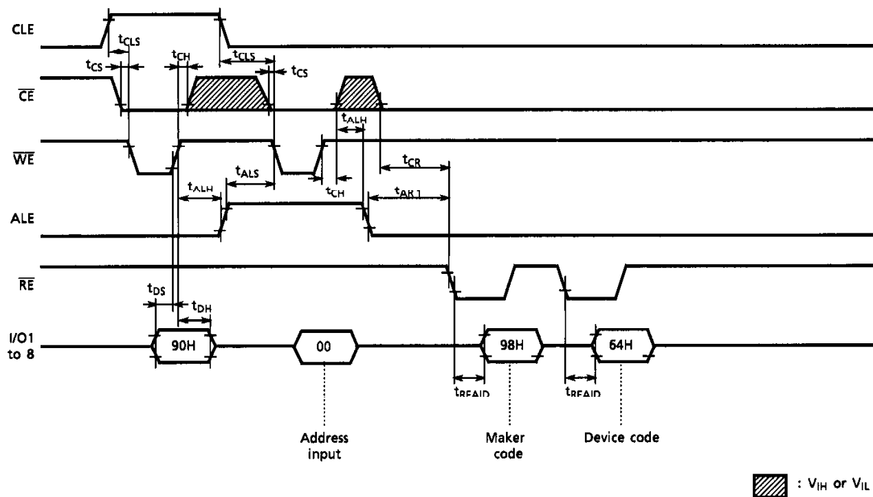
ID Read Operation Timing Diagram
