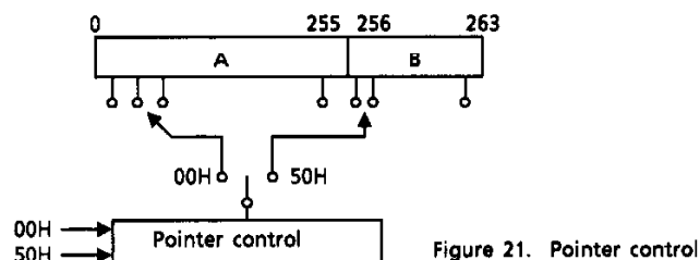
Figure 21. Pointer control
