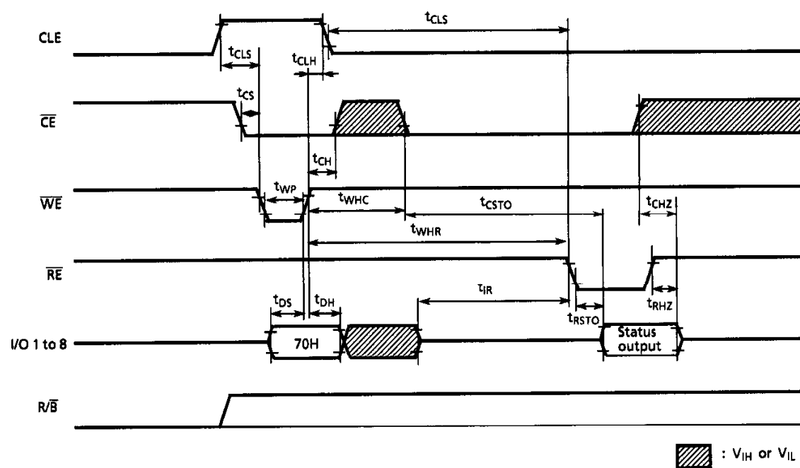
Status Read Cycle Timing Diagram
