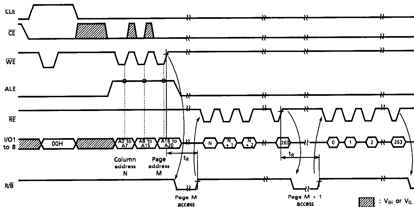
Sequential Read Timing Diagram
