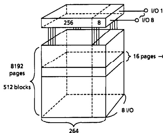
Figure 2. TC58V16 Schematic Cell Layout
