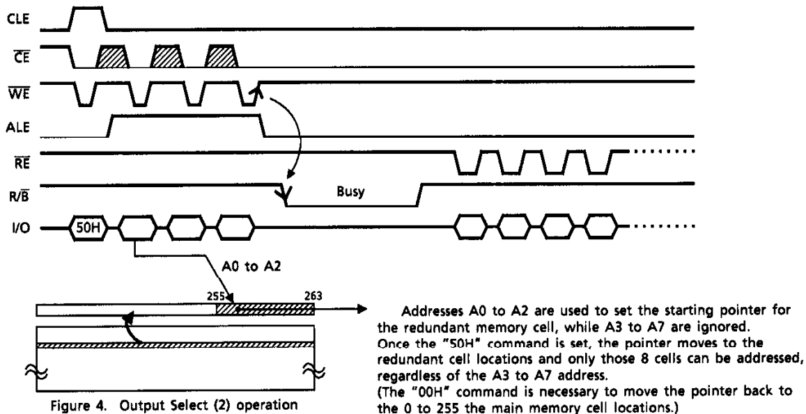
Figure 4. Output Select (2) operation
