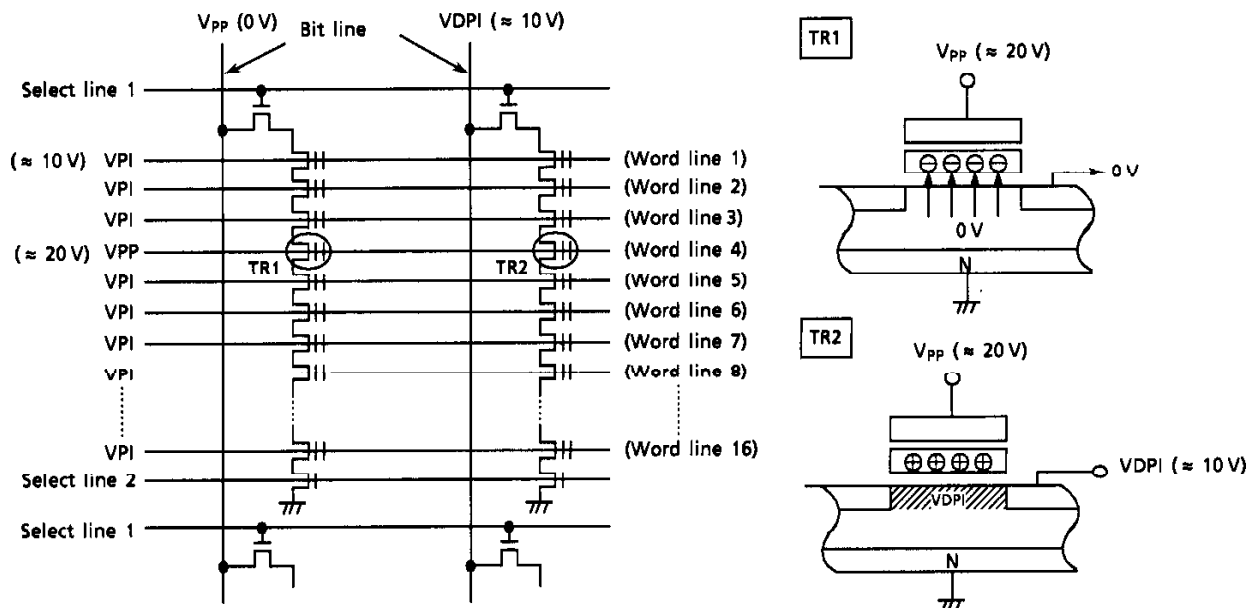
Figure 17. TC5816 Program Device Physics
