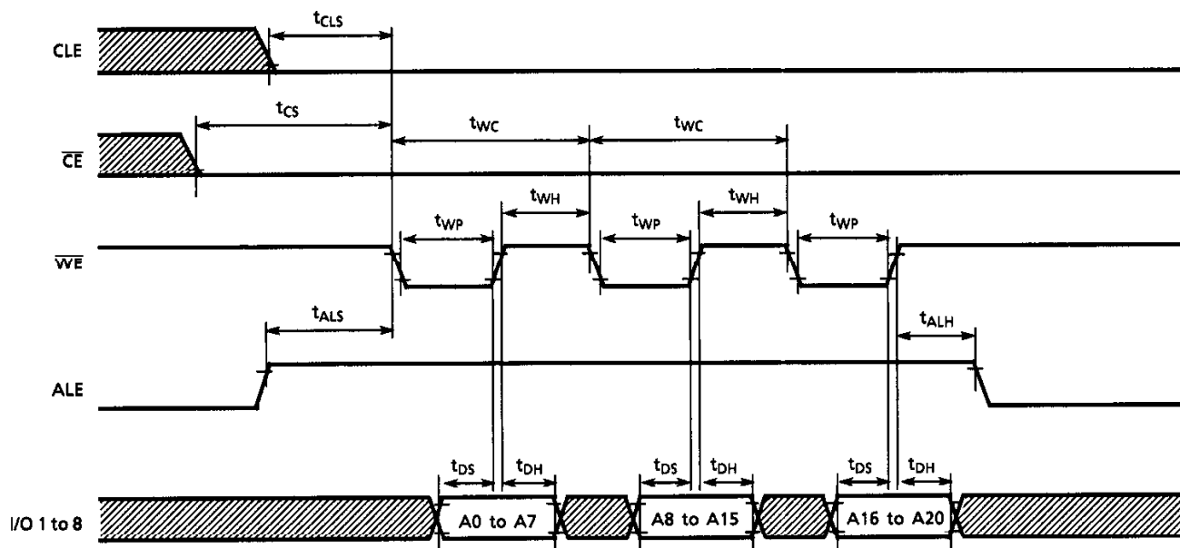
Address Input Cycle Timing Diagram
