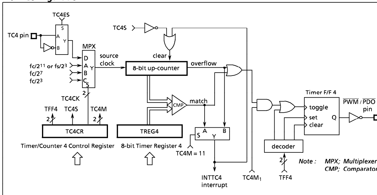
Figure 2-28. Timer/Counter 4
