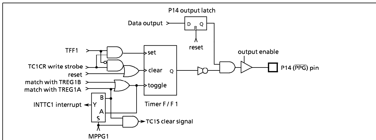
Figure 2-21. PPG Output
