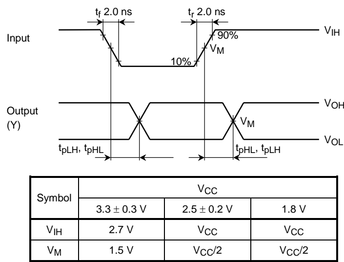
Figure 2 t_{pLH}, t_{pHL}
