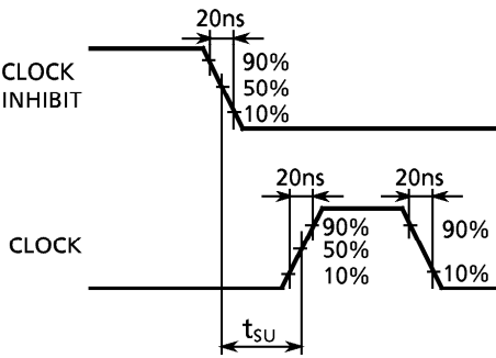
WAVEFORM 3.
