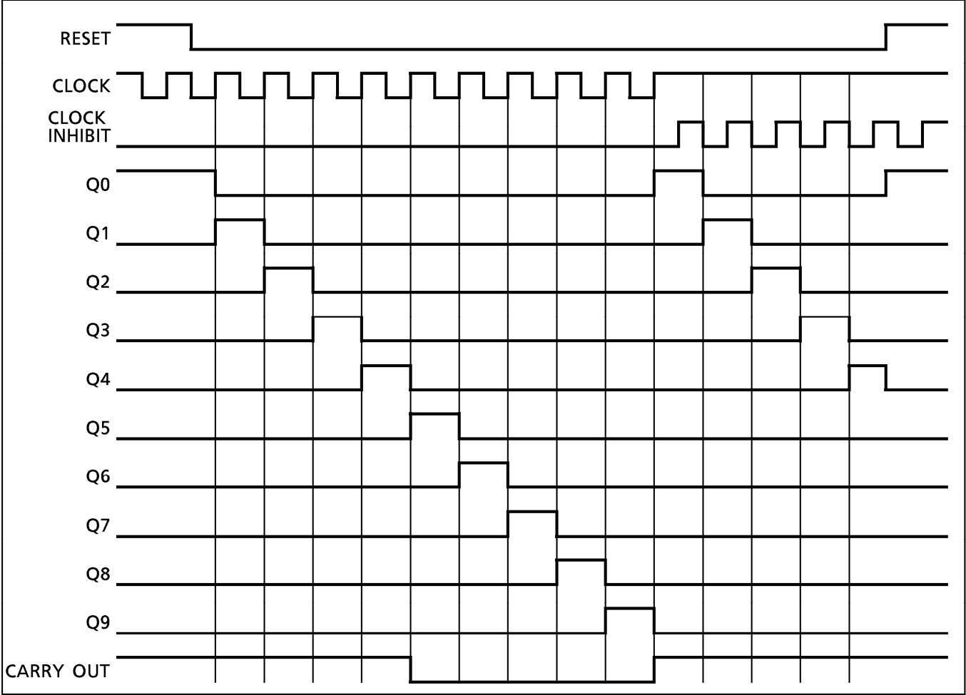
TIMING CHART
