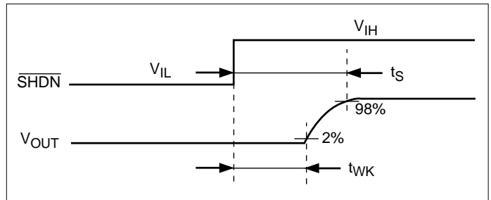
Figure 1: Wake-Up Response Time
