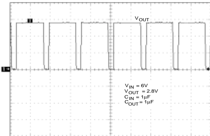
Thermal Shutdown Response
