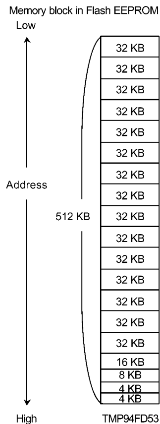
Figure 3.3.1 Block structure of the Flash memory
