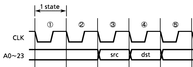
Figure 3.3.2 (1) Micro DMA Cycle Timing
