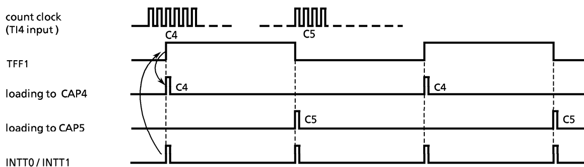
Figure 3.9 (26) Frequency Measurement
