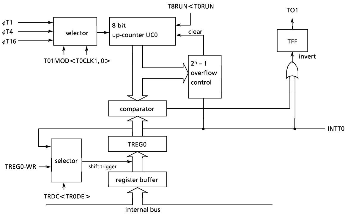
Figure 3.8 (15) 8-Bit PWM Output Mode Block Diagram
