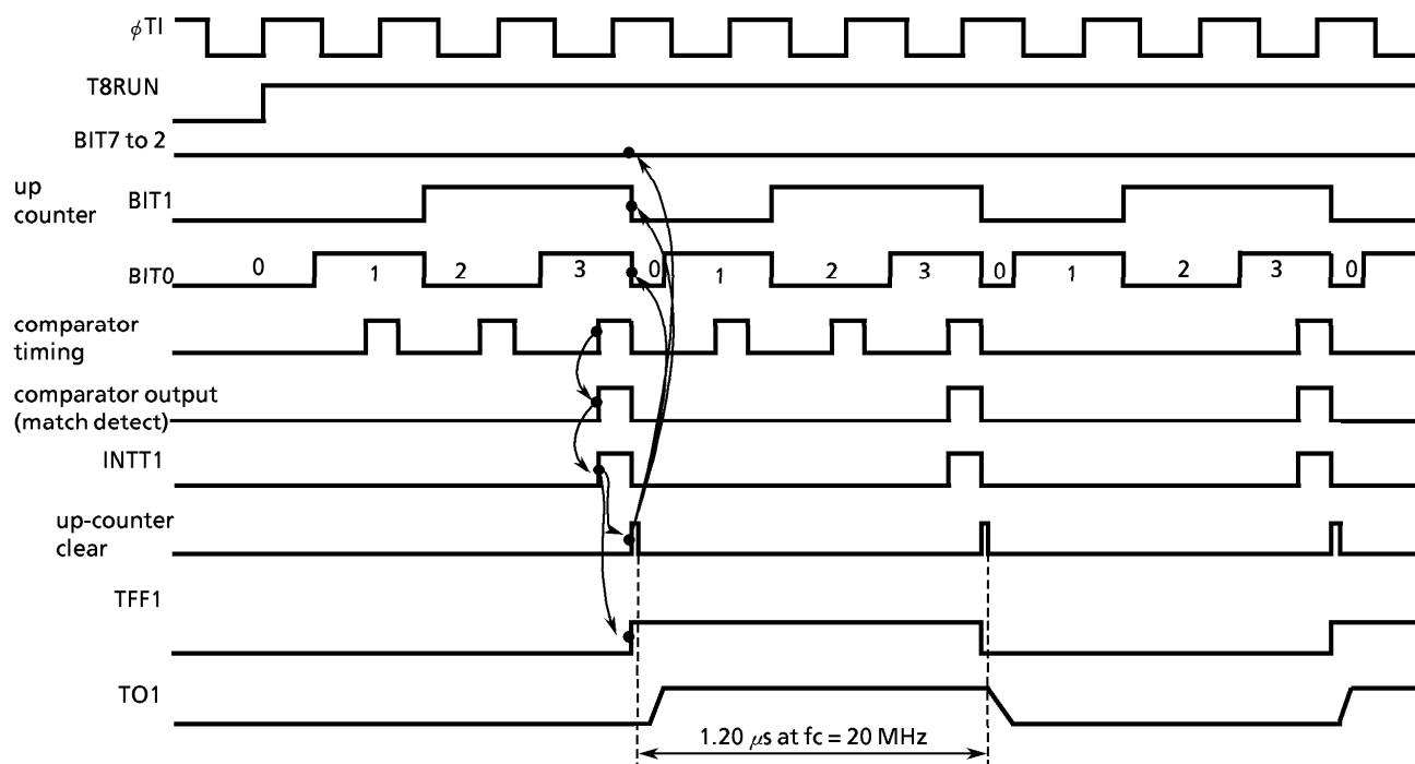
Figure 3.8 (11) Square Wave (50% Duty) Output Timing Chart
