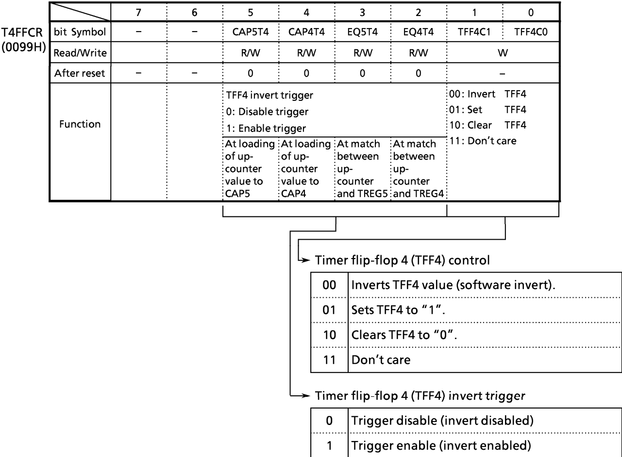
Figure 3.9 (7) 16-Bit Timer 4 F/F Control (T4FFCR)
