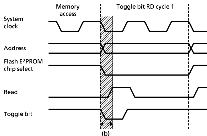
Figure 3.6 (3) Flash E 2 PROM Toggle Bit Read cycle
