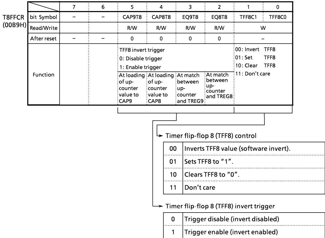
Figure 3.9 (13) 16-Bit Timer 8 F/F Control (T8FFCR)
