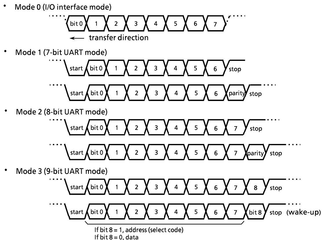
Figure 3.10 (1) Data Formats
