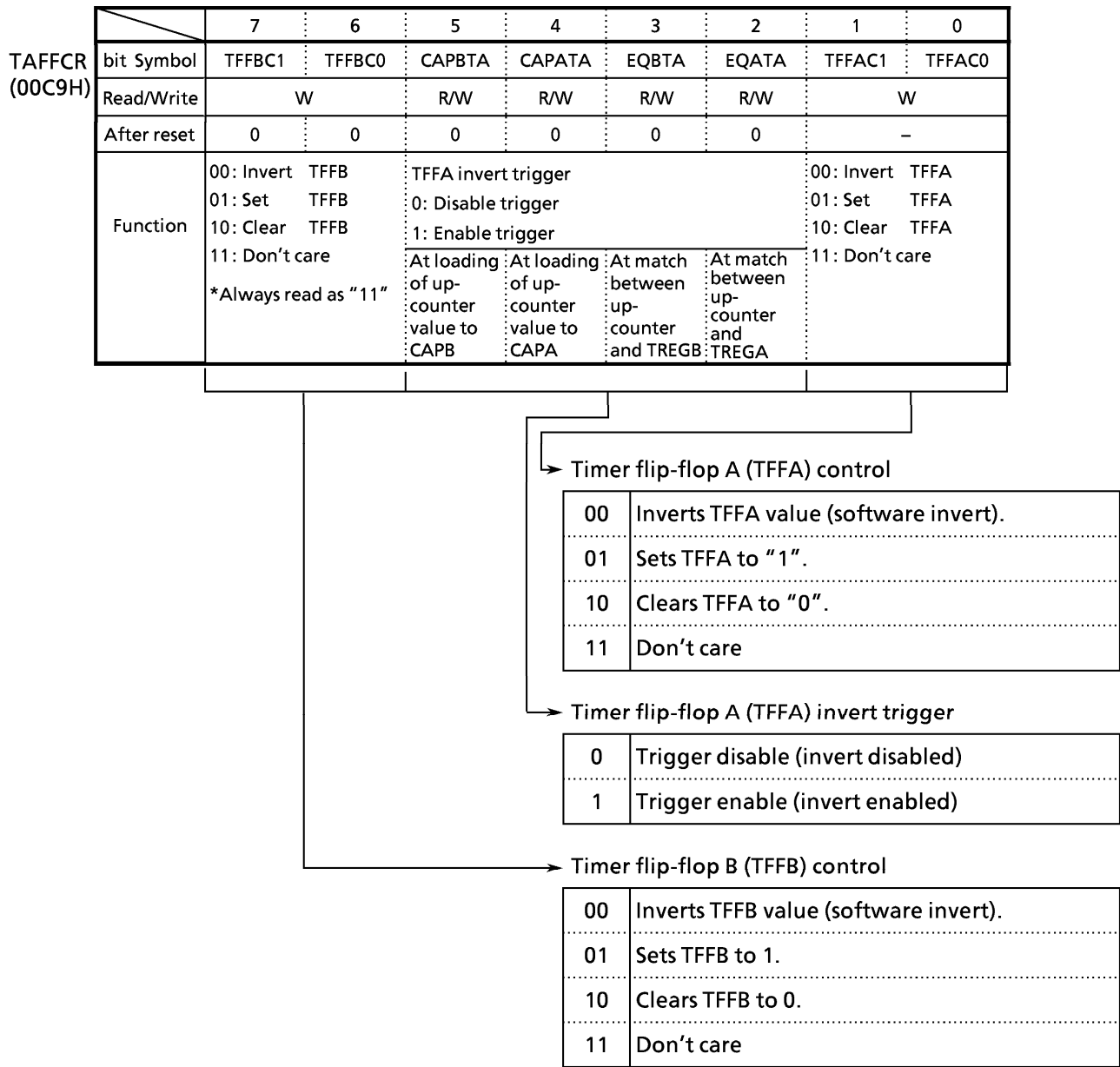
Figure 3.9 (16) 16-Bit Timer A F/F Control (TAFFCR)
