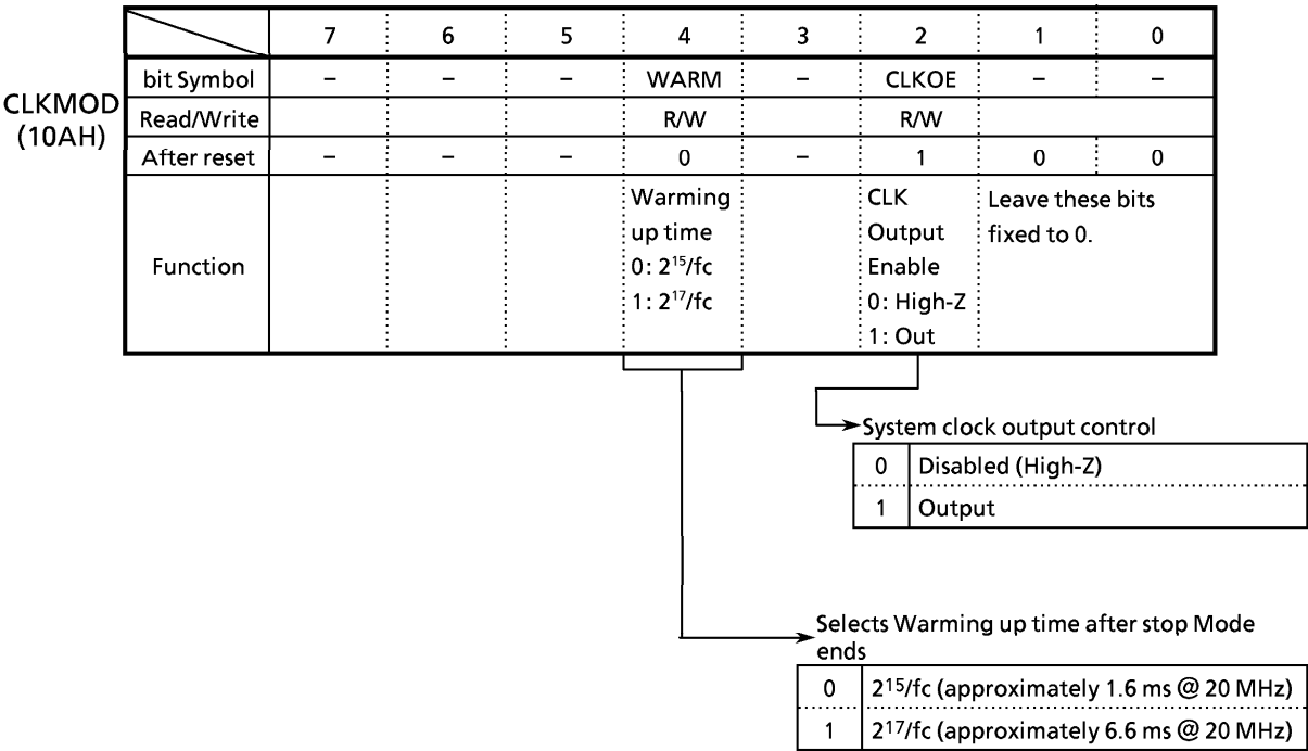
Figure 3.13 (5) CLOCK Mode Register
