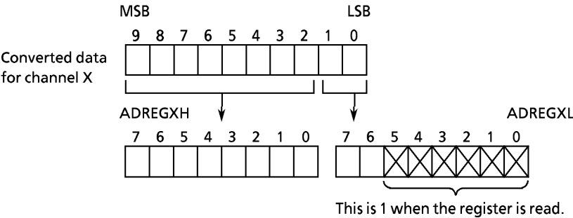
図3.11 (3-2) AD Conversion Result Register (ADREG26, 37)
