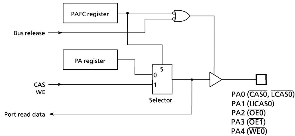
Figure 3.5 (10) Port A
