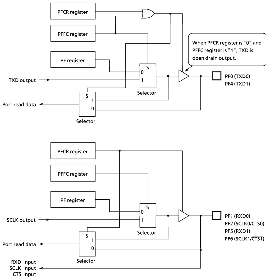
Figure 3.5 (15) Port F
