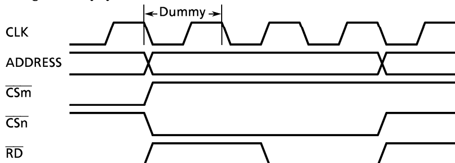
Figure 3.6 (1) Read Cycle when Dummy Cycle is Inserted
