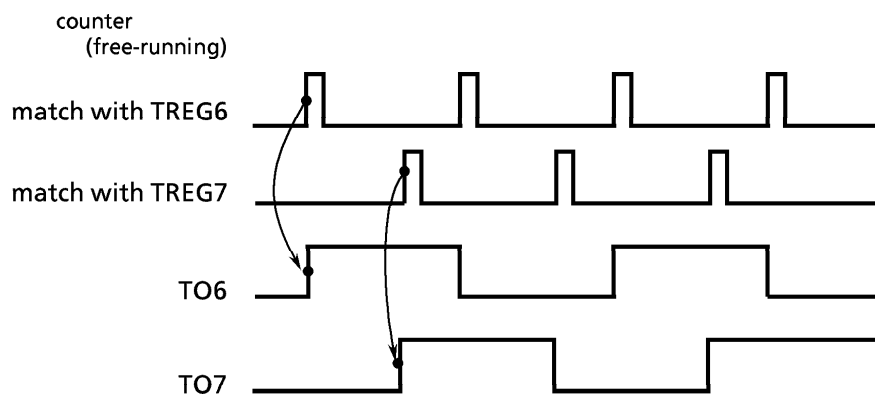
Figure 3.9 (29) Phase Output
