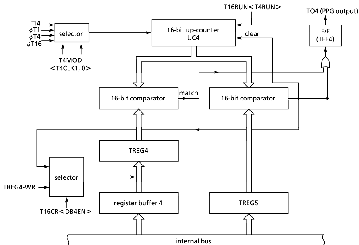
Figure 3.9 (23) 16-Bit PPG Mode Block Diagram
