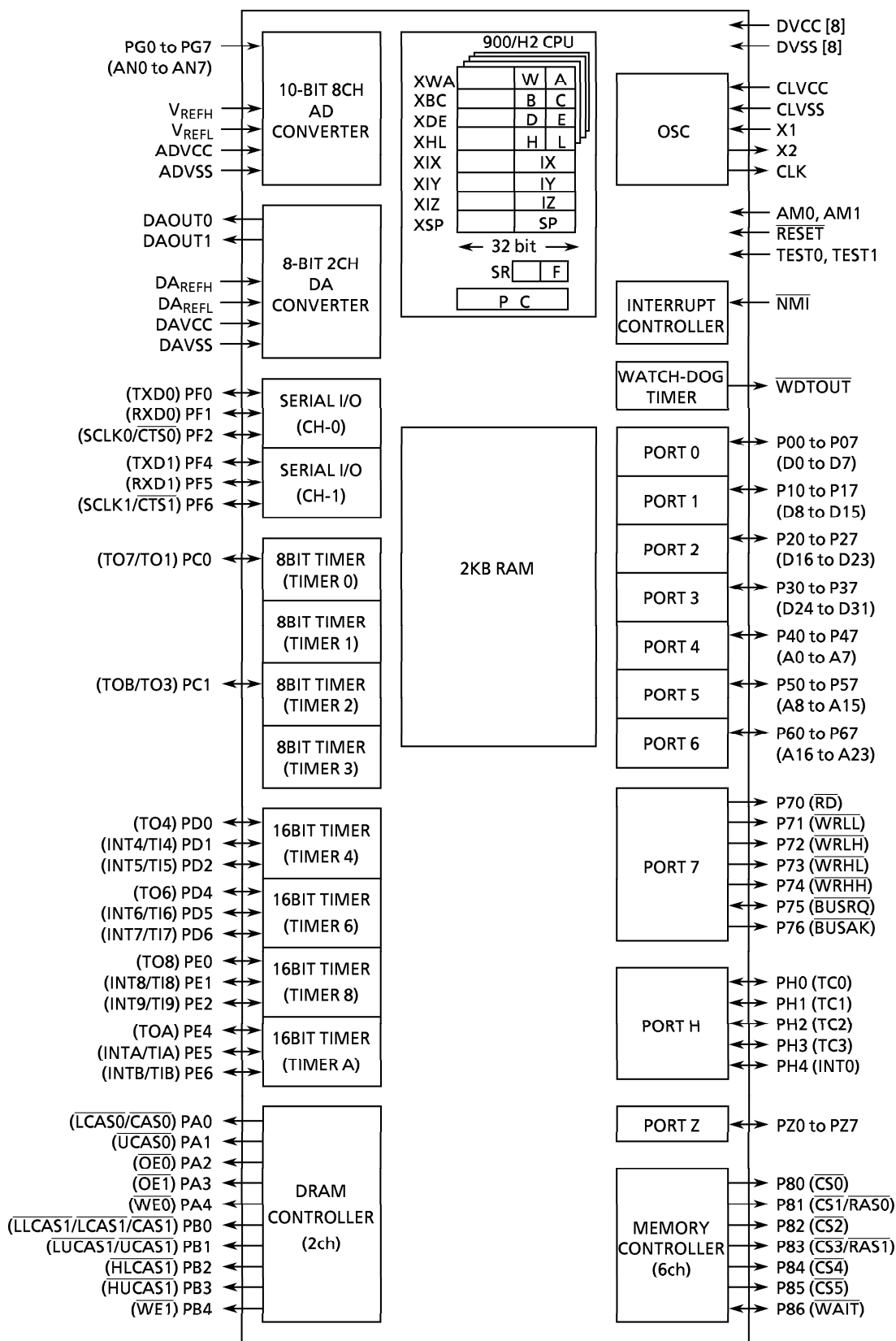
Figure 1 TMP94C241C Block Diagram
