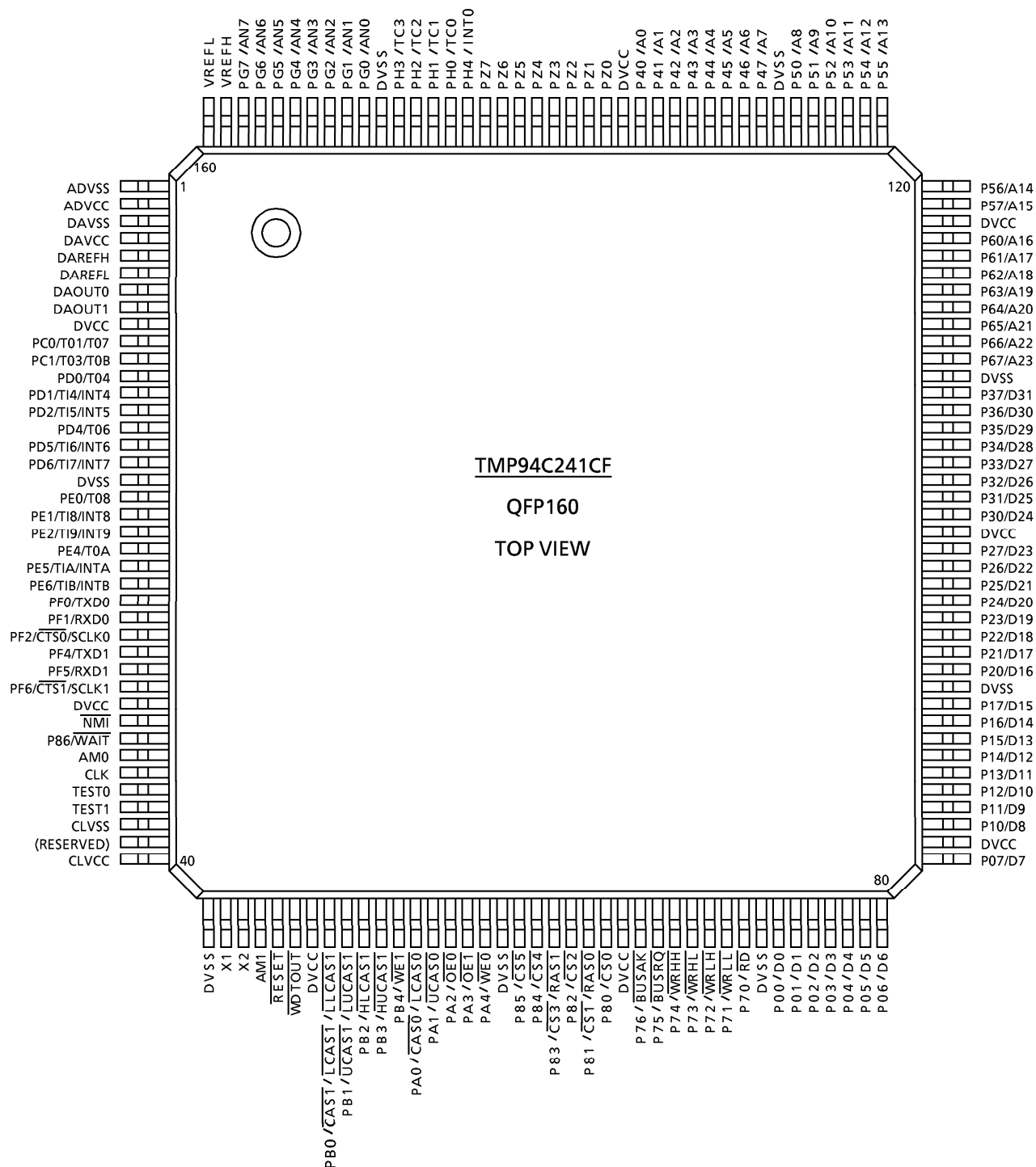
Figure 2.1 Pin Assignment
