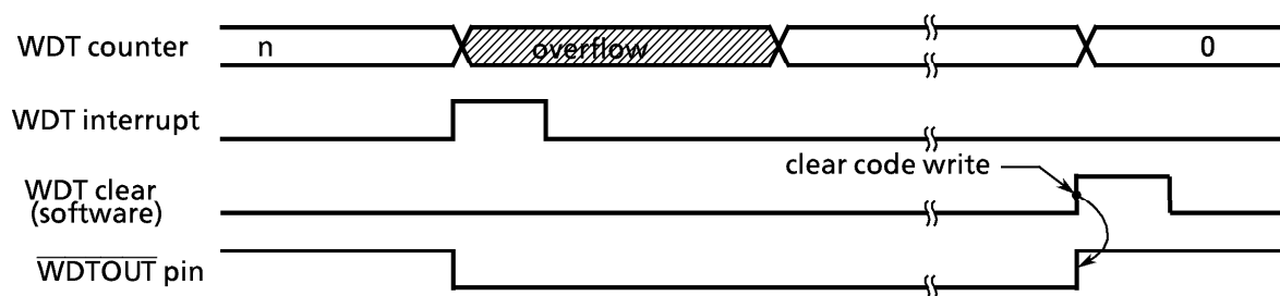
Figure 3.13 (2) Watchdog Timer Output During Overflow
