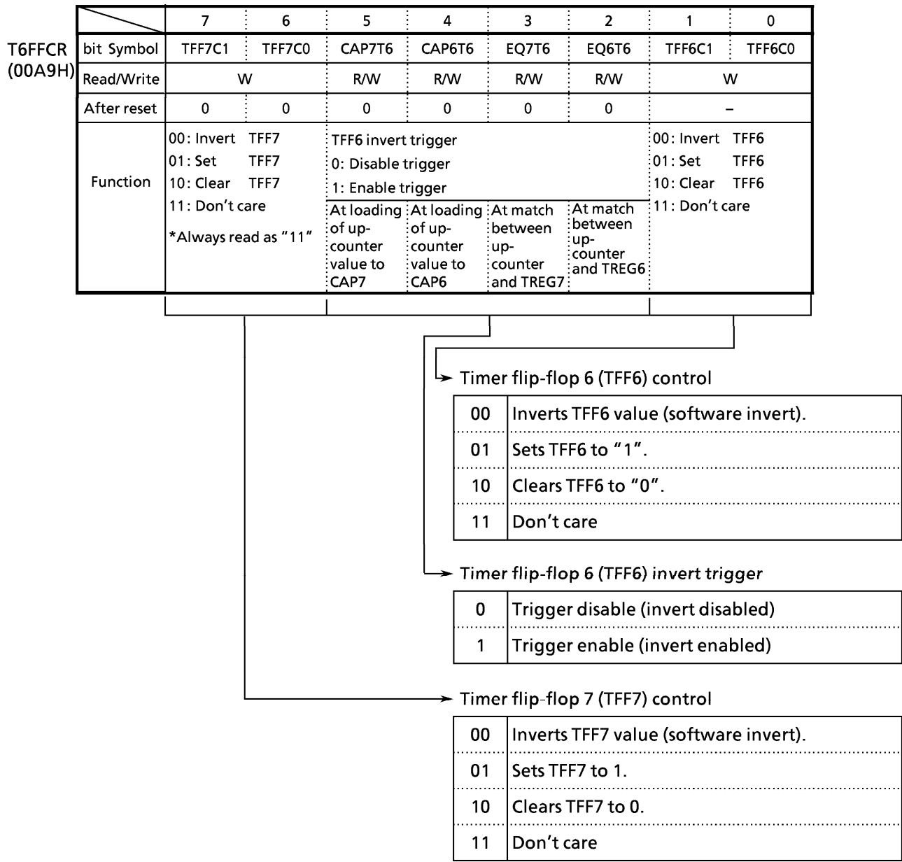
Figure 3.9 (10) 16-Bit Timer 6 F/F Control (T6FFCR)
