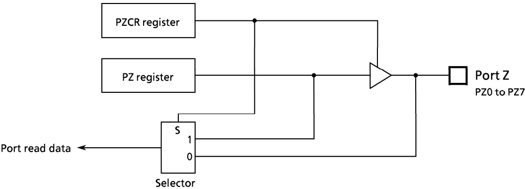
Figure 3.5 (18) Port Z
