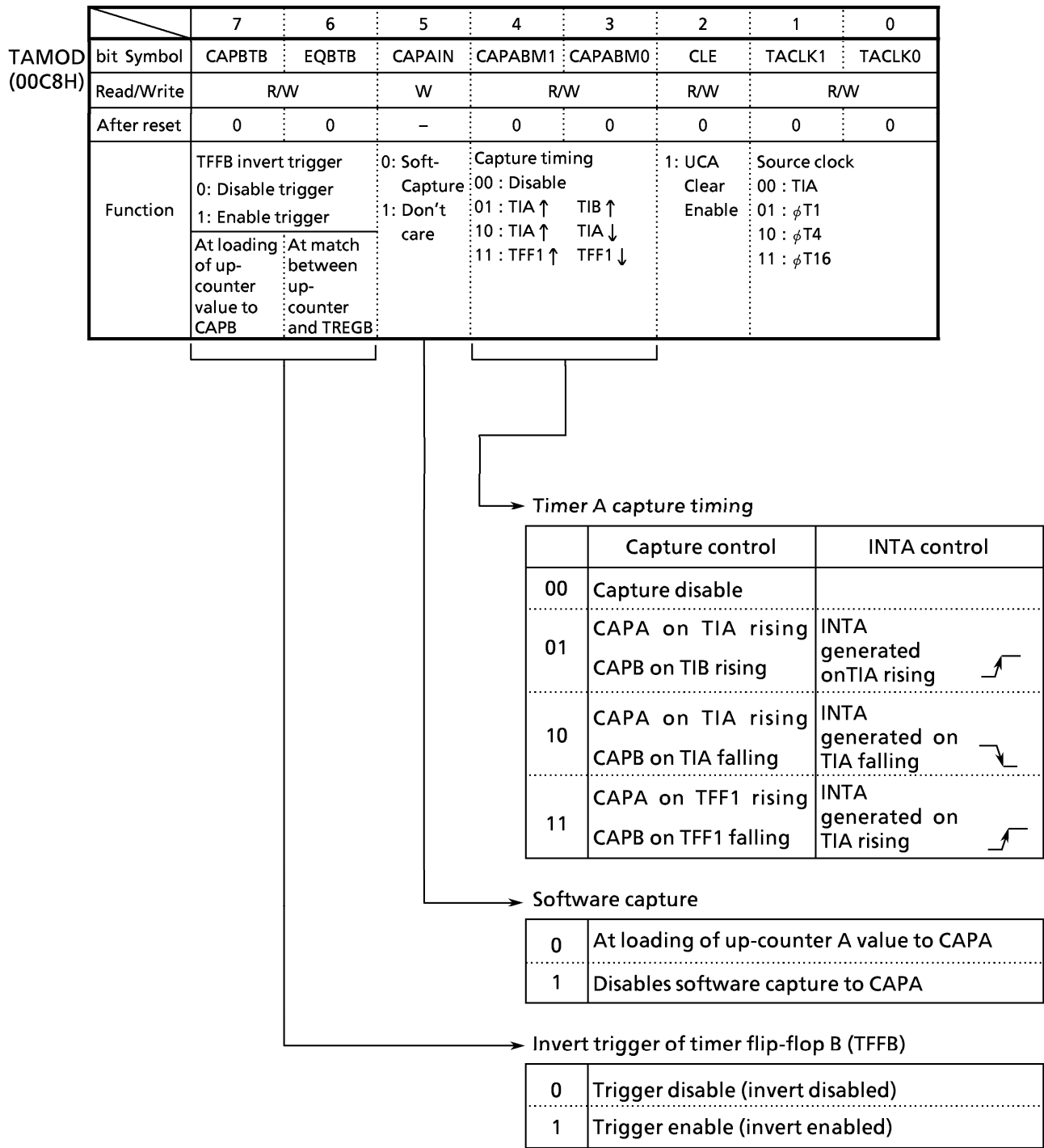
Figure 3.9 (15) 16-Bit Timer Control Register (TAMOD) (2/2)
