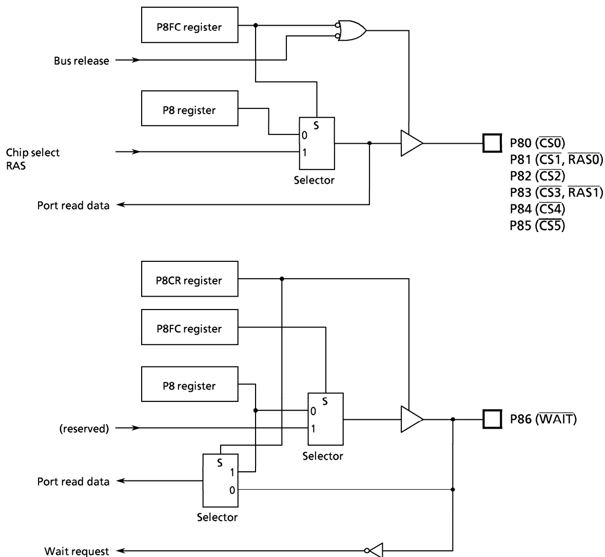
Figure 3.5 (9) Port 8
