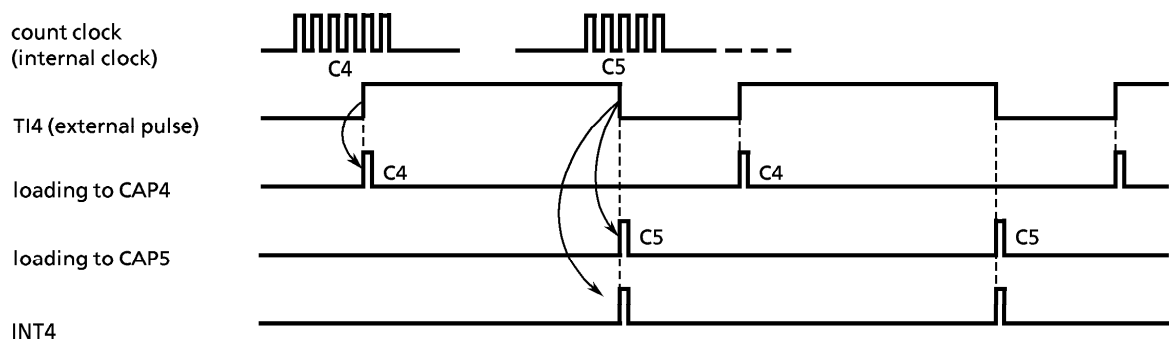
Figure 3.9 (27) Pulse Width Measurement
