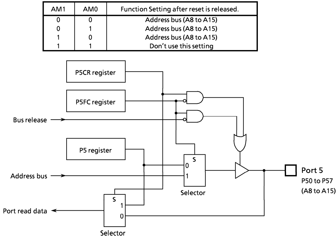
Figure 3.5 (6) Port 5
