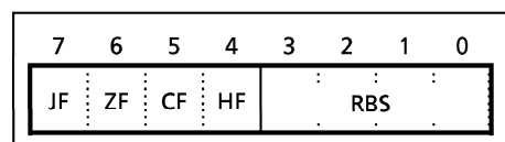
Figure 1-6. PSW (Flags, RBS) Configuration
