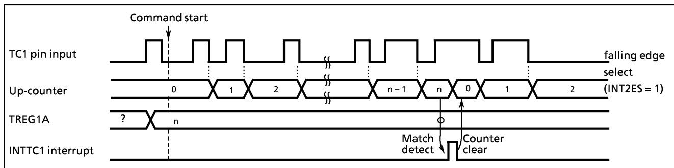
Figure 2-14. Event Counter Mode Timing Chart
