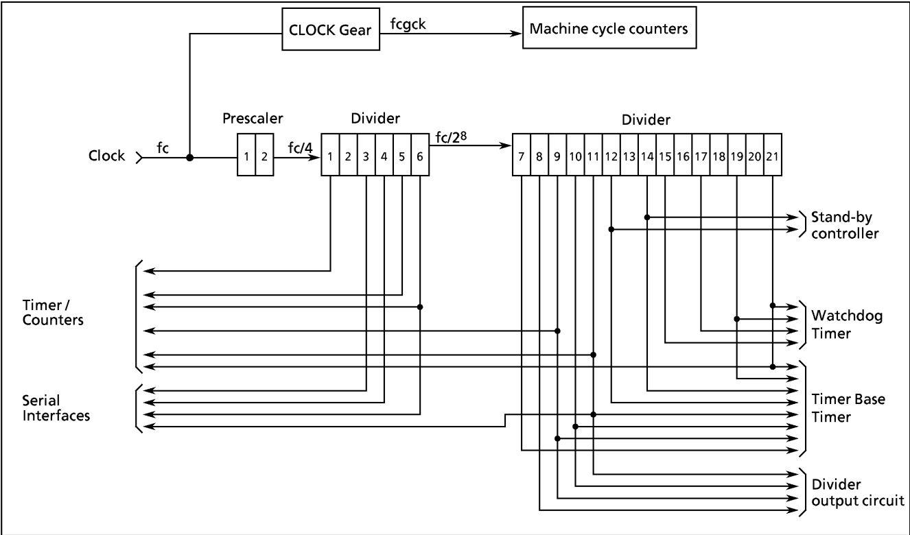
Figure 1-14. Configuration of Timing Generator
