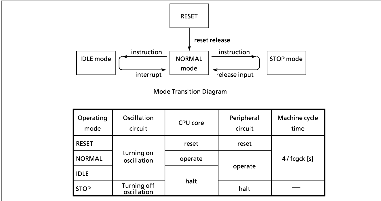
Figure 1-16. Operating Mode Transition Diagram
