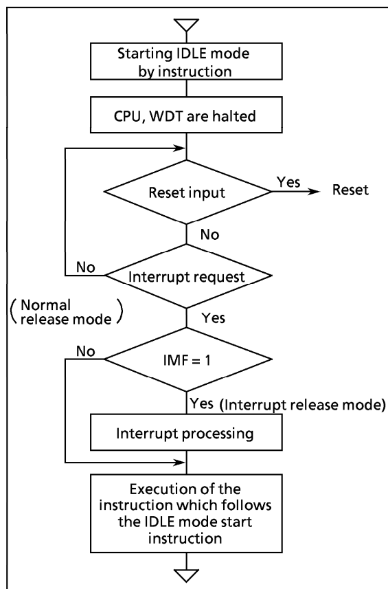
Figure 1-21. IDLE Mode
