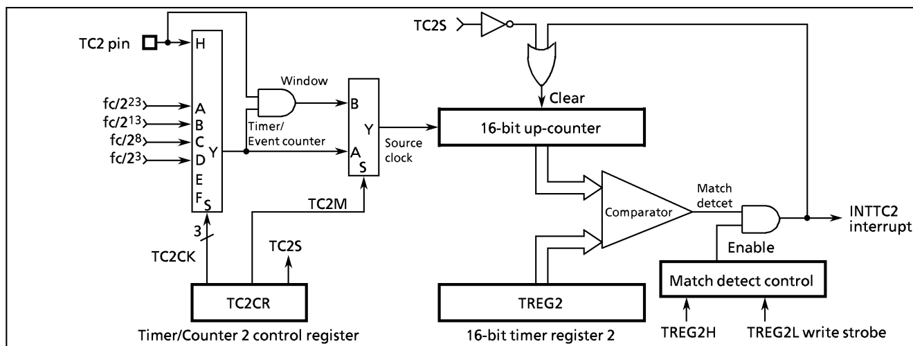
Figure 2-19. Timer/Counter 2 (TC2)
