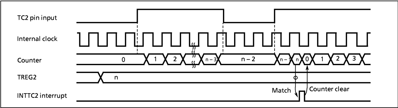
Figure 2-21. Window Mode Timing Chart
