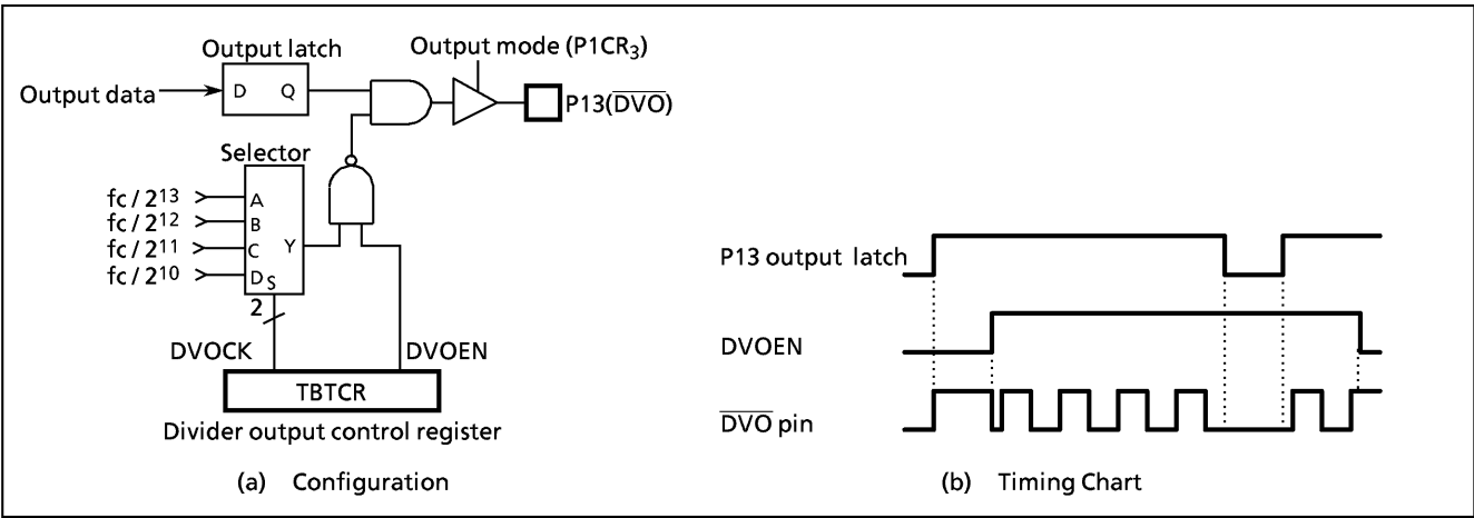
Figure 2-9. Divider Output
