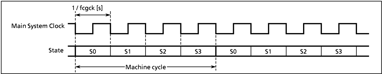
Figure 1-15. Machine Cycle
