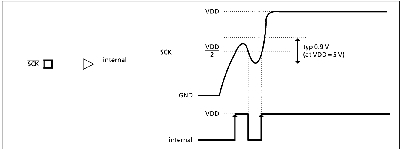
Figure 2-33. Example of ringing noise
