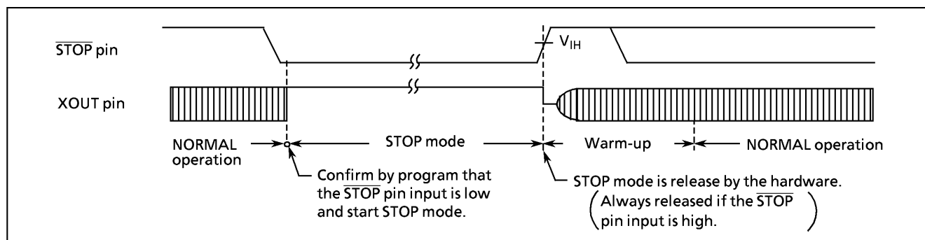
Figure 1-18. Level Mode
