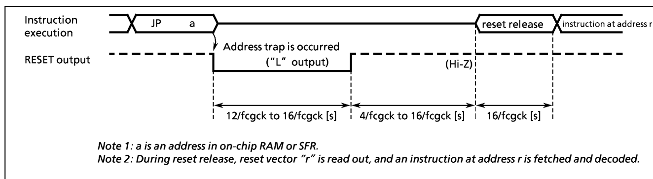
Figure 1-32. Address Trap Reset
