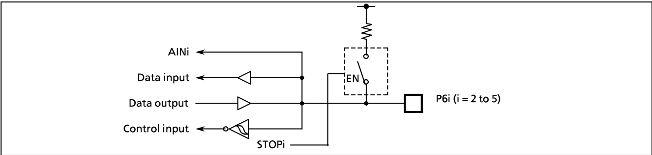
Figure 2-42. Port P6i (i = 2 to 5)
