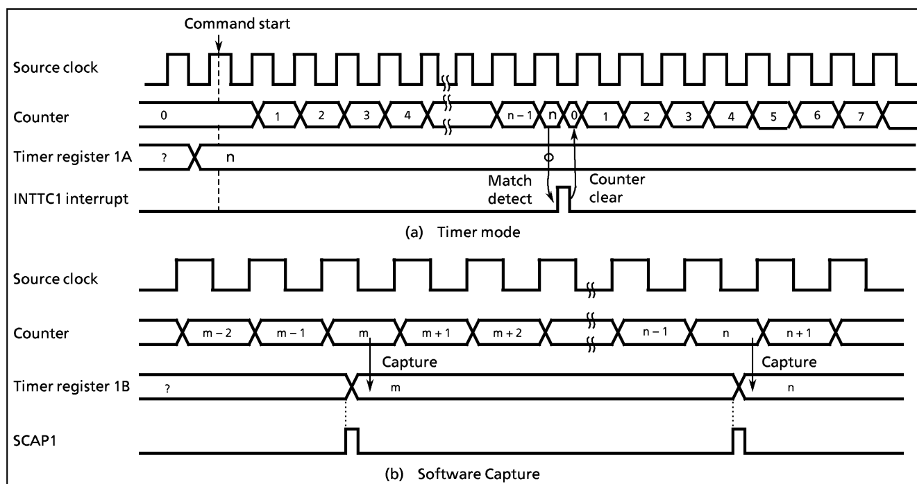
Figure 2-12. Timer Mode Timing Chart
