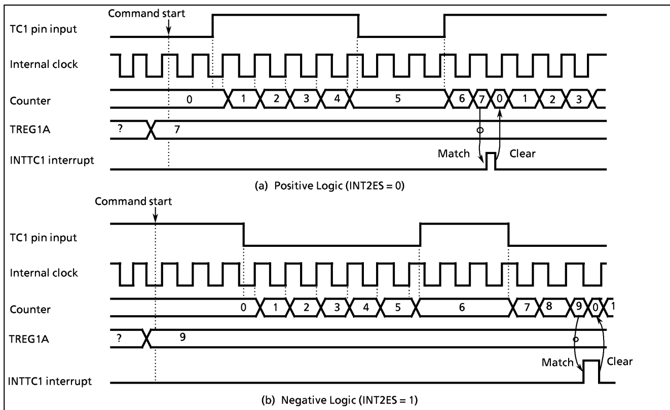
Figure 2-15. Window Mode Timing Chart
