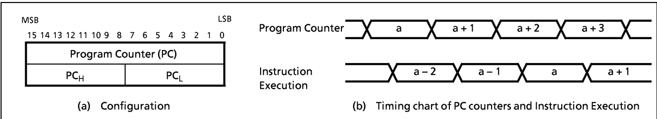
Figure 1-3. Program Counter
