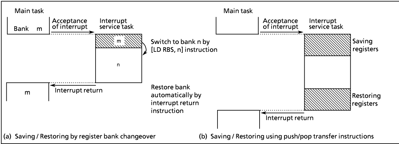
Figure 1-26. Saving / Restoring General-purpose Registers
