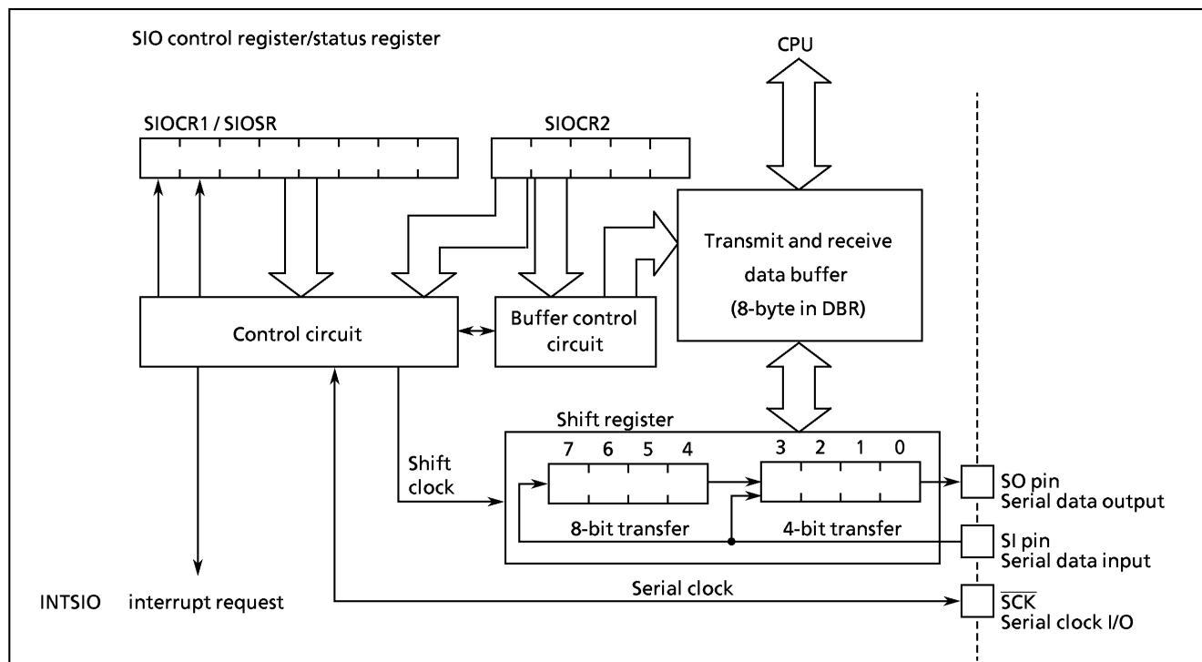
Figure 2-22. Serial Interface
