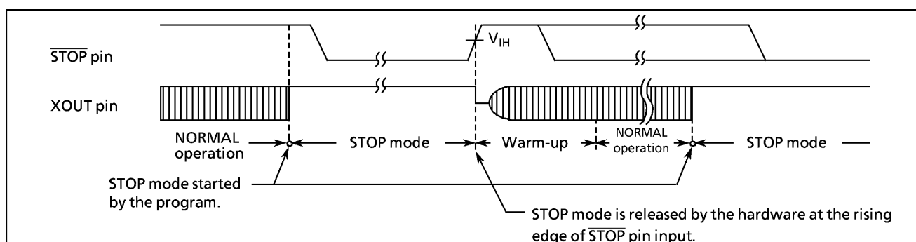
Figure 1-19. Edge-sensitive Mode
