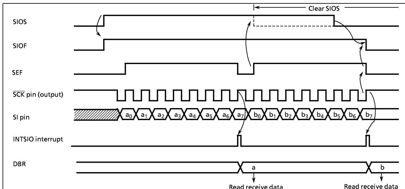
Figure 2-30. Receive Mode (Example: 8-bit, 1 word, internal clock)
