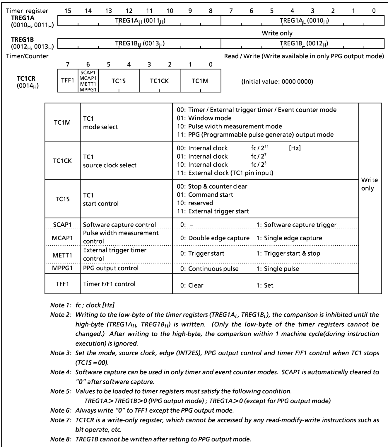
Figure 2-11. Timer Registers and Control Register TC1
