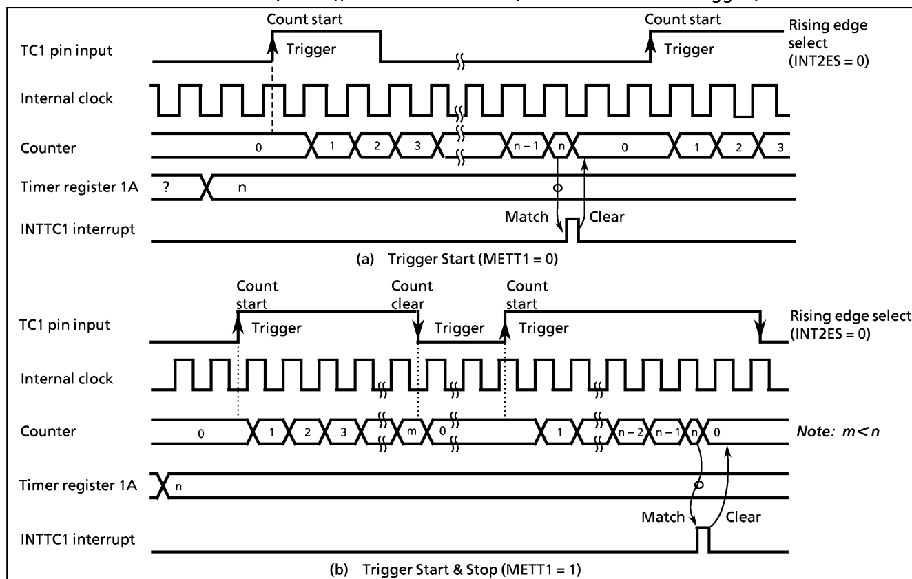
Figure 2-13. External Trigger Timer Mode Timing Chart
