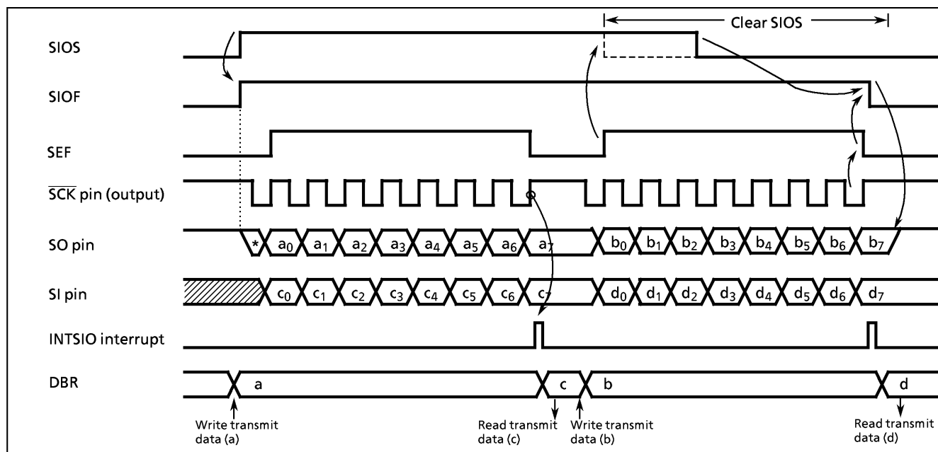
Figure 2-31. Transmit/Receive Mode (Example: 8-bit, 1 word, internal clock)
