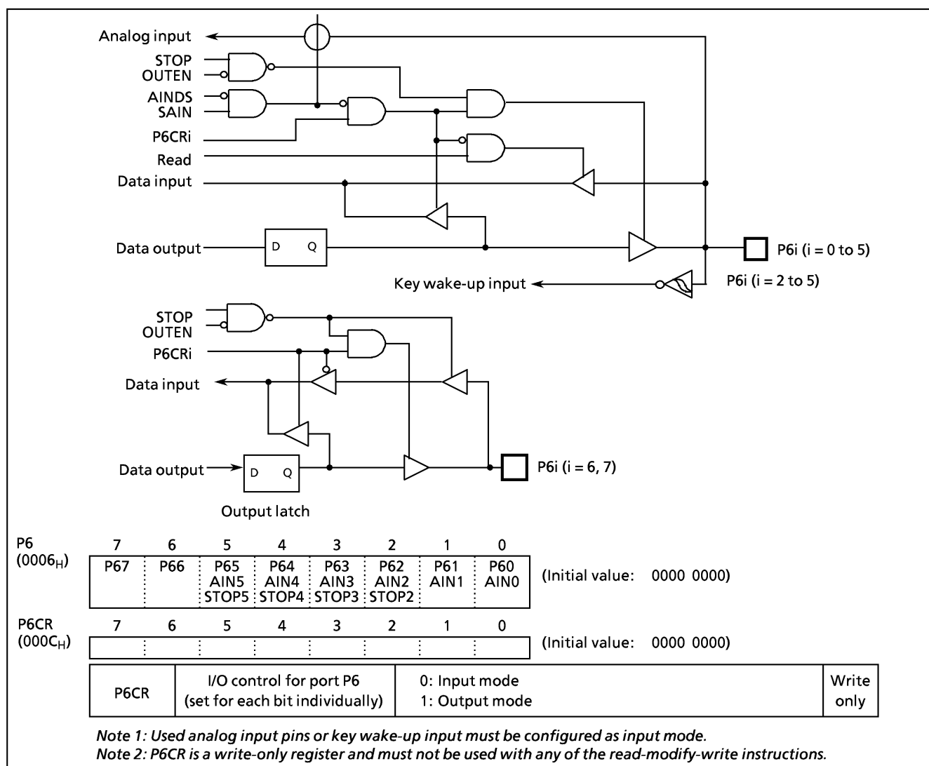
Figure 2-4. Port P6 and P6CR
