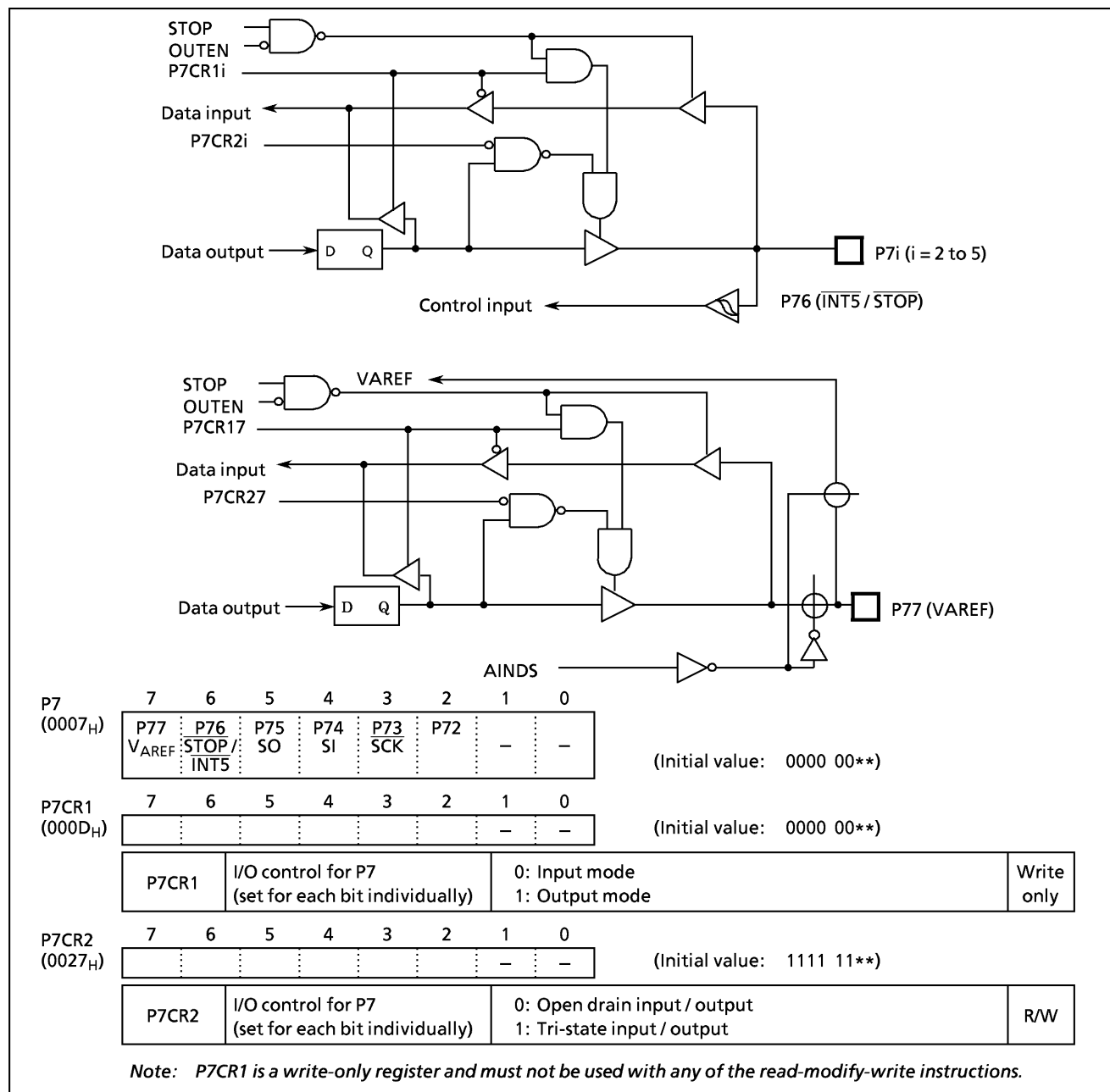
Figure 2-5. Port P7 and P7CR
