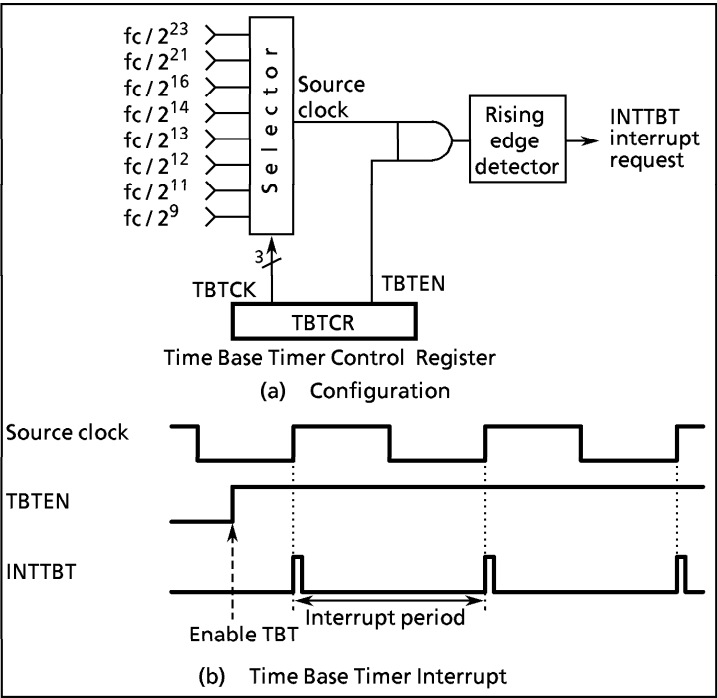
Figure 2-6. Time Base Timer
