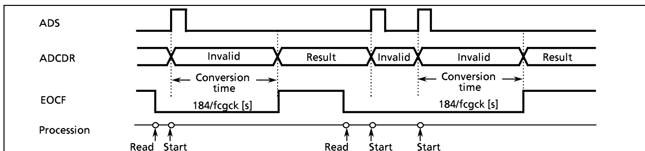
Figure 2-38. A/D Conversion Timing Chart (ACK = 0)
