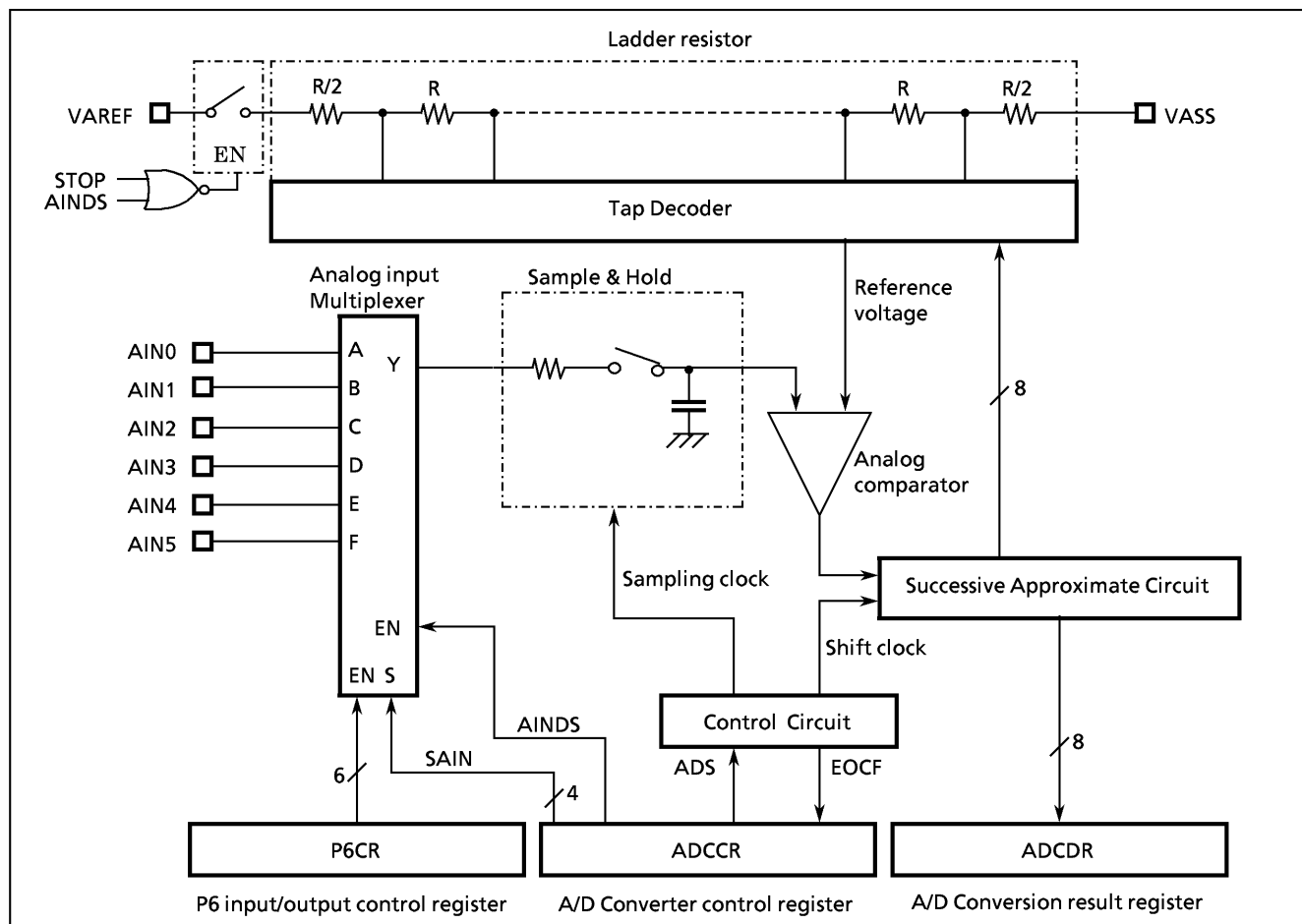
Figure 2-35. A/D Converter (ADC)
