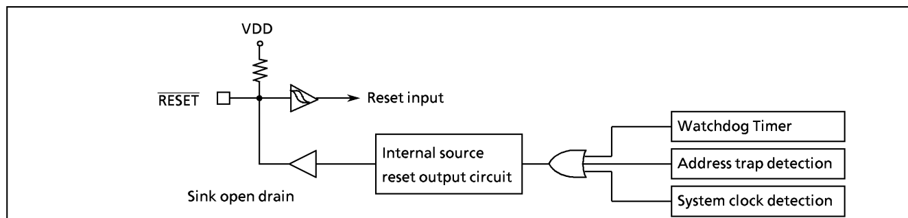
Figure 1-31. Reset Circuit
