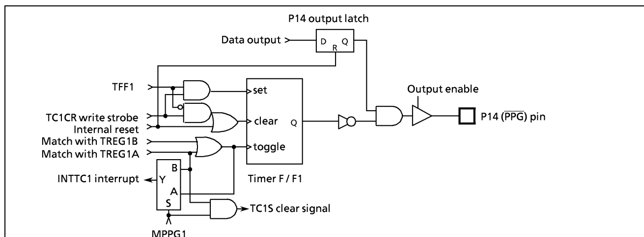
Figure 2-17. \overline{\text{PPG}} Output
