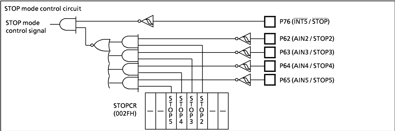
Figure 2-41. Stop Mode Control Circuit
