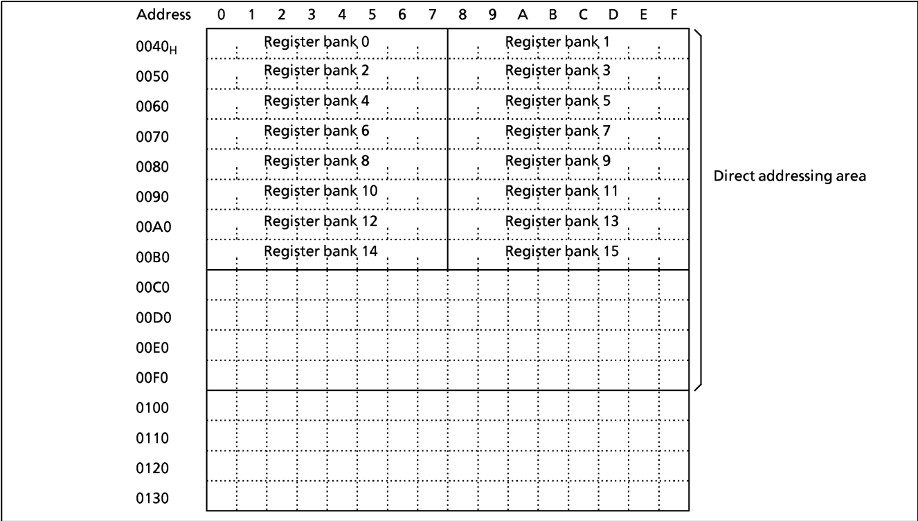
Figure 1-4. Data Memory Map
