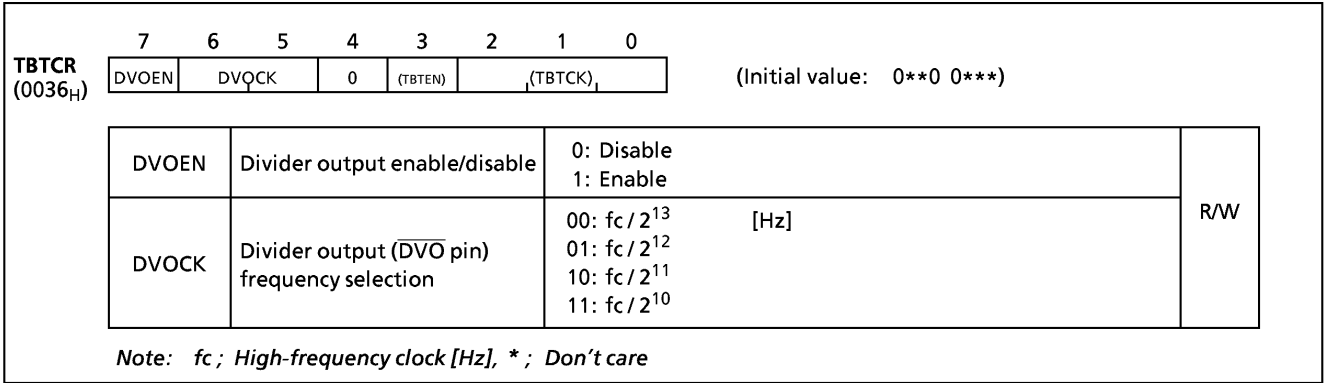
Figure 2-8. Divider Output Control Register
