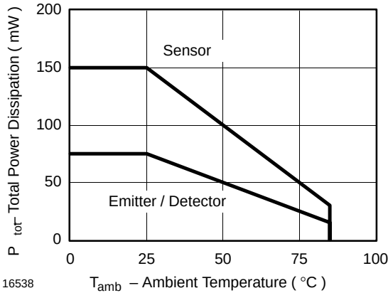
Figure 1. Derating diagram
